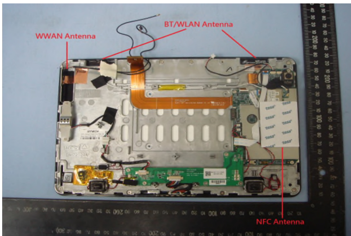
BT / WLAN / WWAN / NFC Antenna
