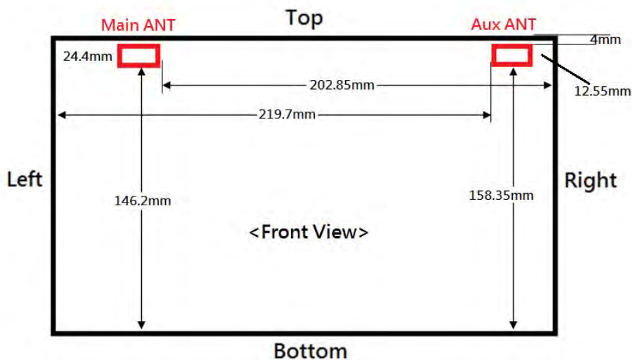
Fig.9 Antenna location
