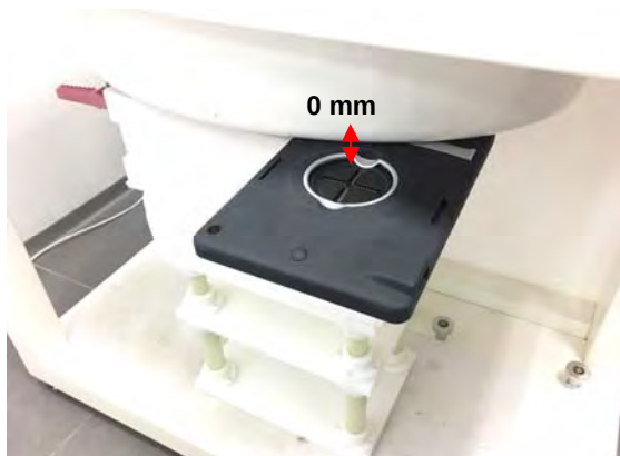
Fig.3 EUT Back side_Main to flat phantom
