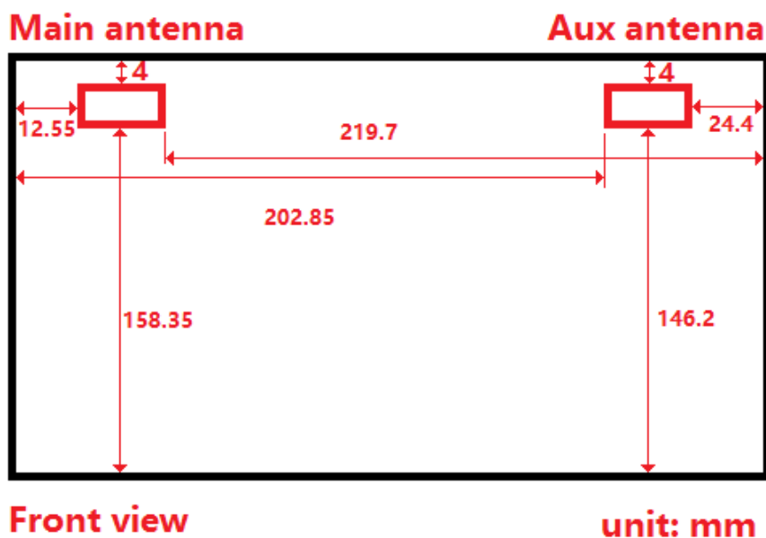
Fig.11 Antenna location
