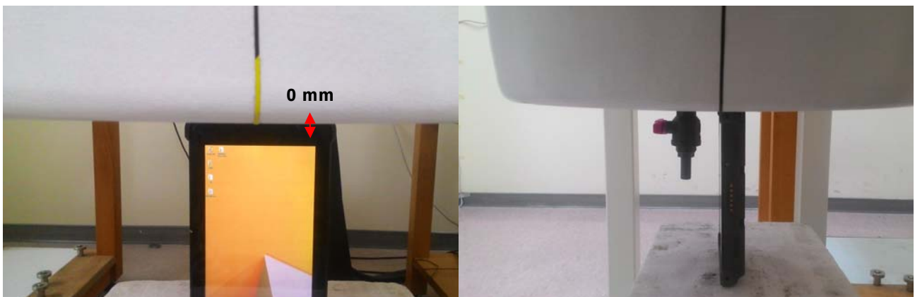
Fig.5 EUT Right side to flat phantom
