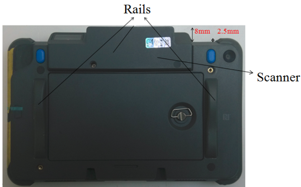
Fig.9 Back view of EUT(with scanner and rails)
