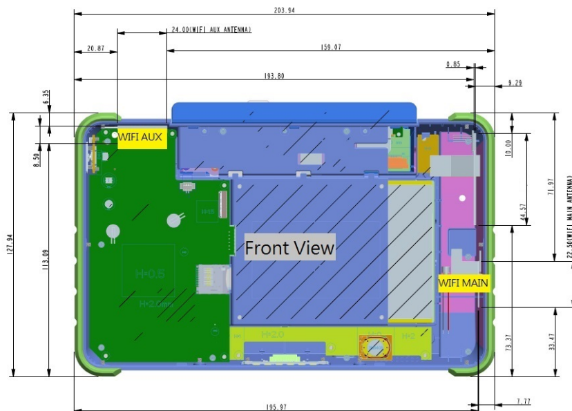
Fig.11 Antenna position of EUT (Front view)
