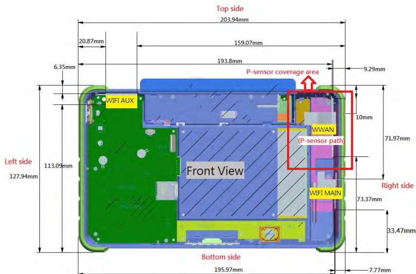
Fig.13 Antenna position of EUT (Front view)
