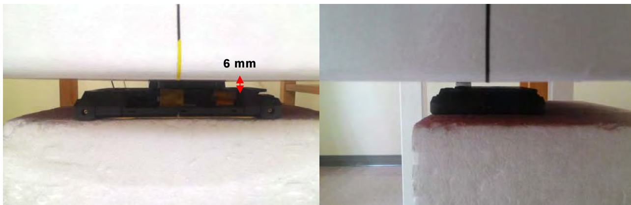
Fig.7 EUT back side to flat phantom
