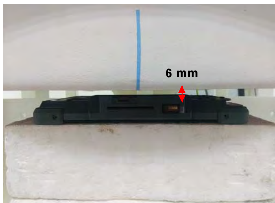
Fig.6 EUT back side to flat phantom
