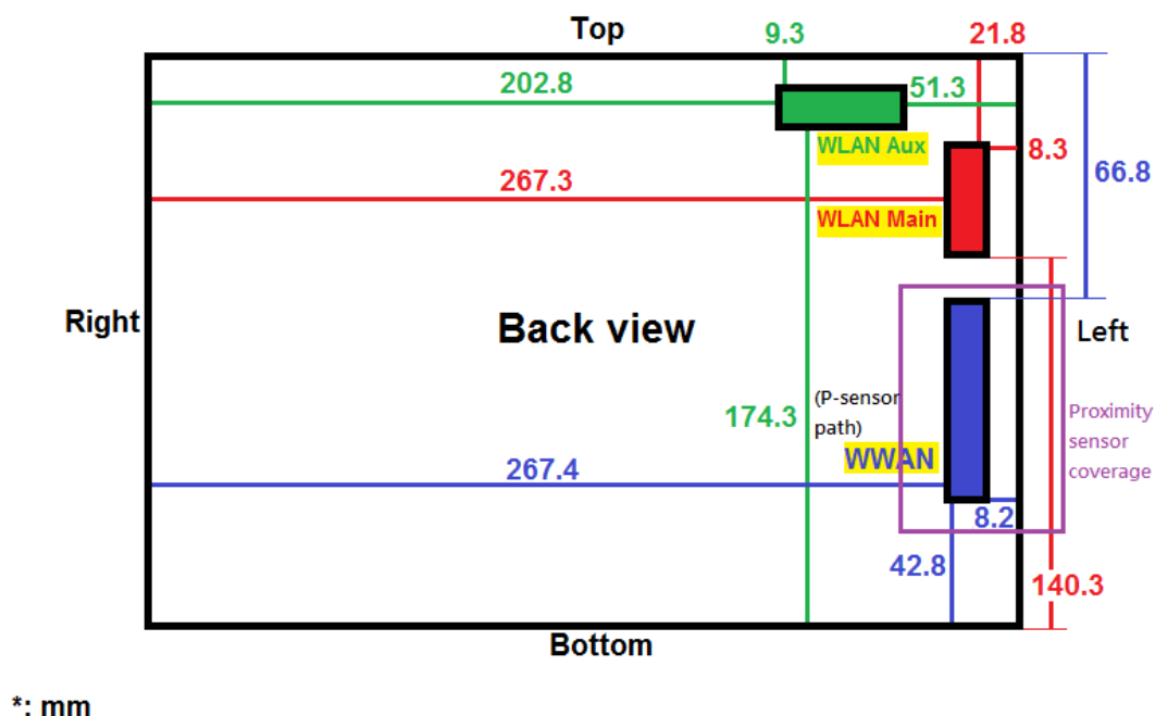
Fig.11 Antenna position of EUT
