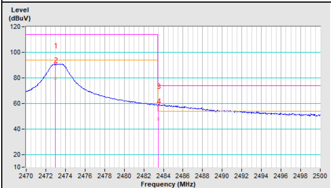
2473MHz Vertical
