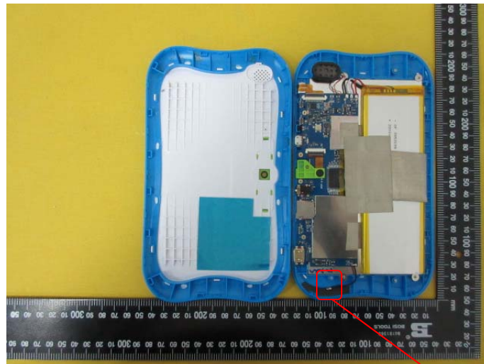
WIFI/BT Antenna
