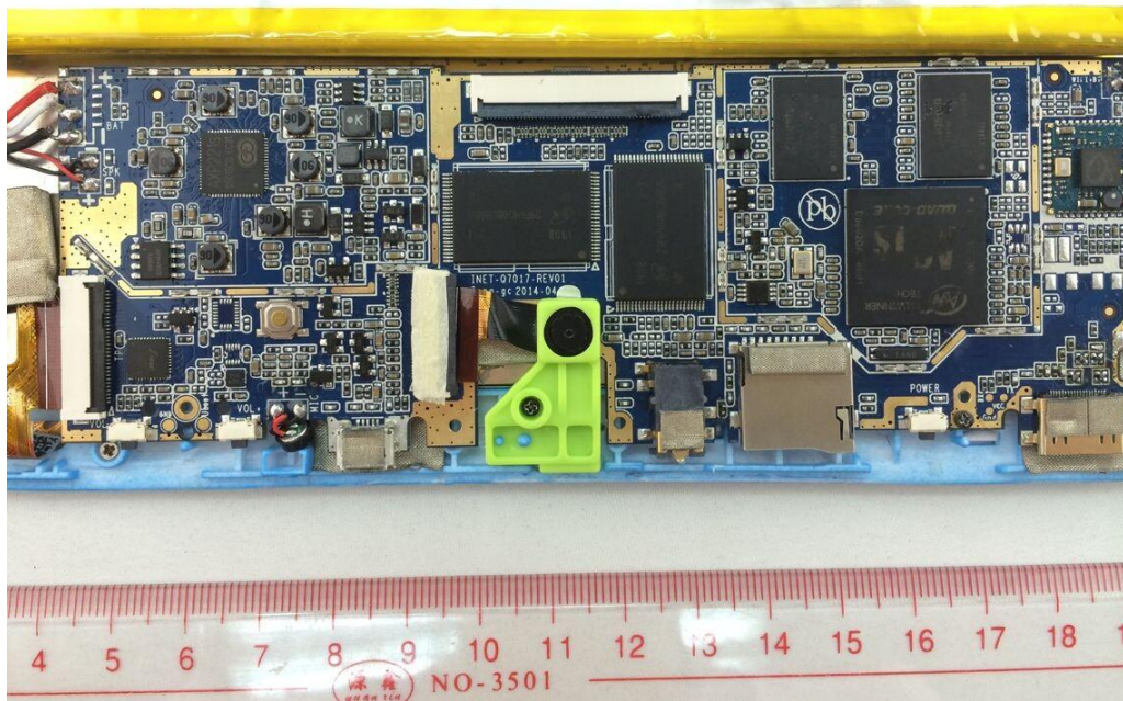
MAIN BOARD TOP VIEW 3
