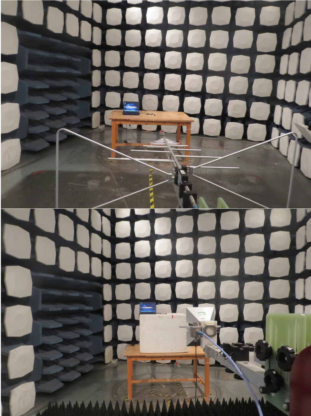
Picture 1 Radiated Spurious Emissions Test setup
