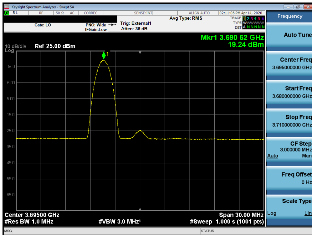
Plot 7-75. Peak Power Spectral Density Plot (B48 – 10.0MHz 64-QAM – High Channel RB: 1 RB, Offset: 0)
