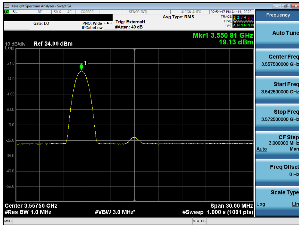
Plot 7-76. Peak Power Spectral Density Plot (B48 – 15.0MHz QPSK – Low Channel RB: 1 RB, Offset: 0)
