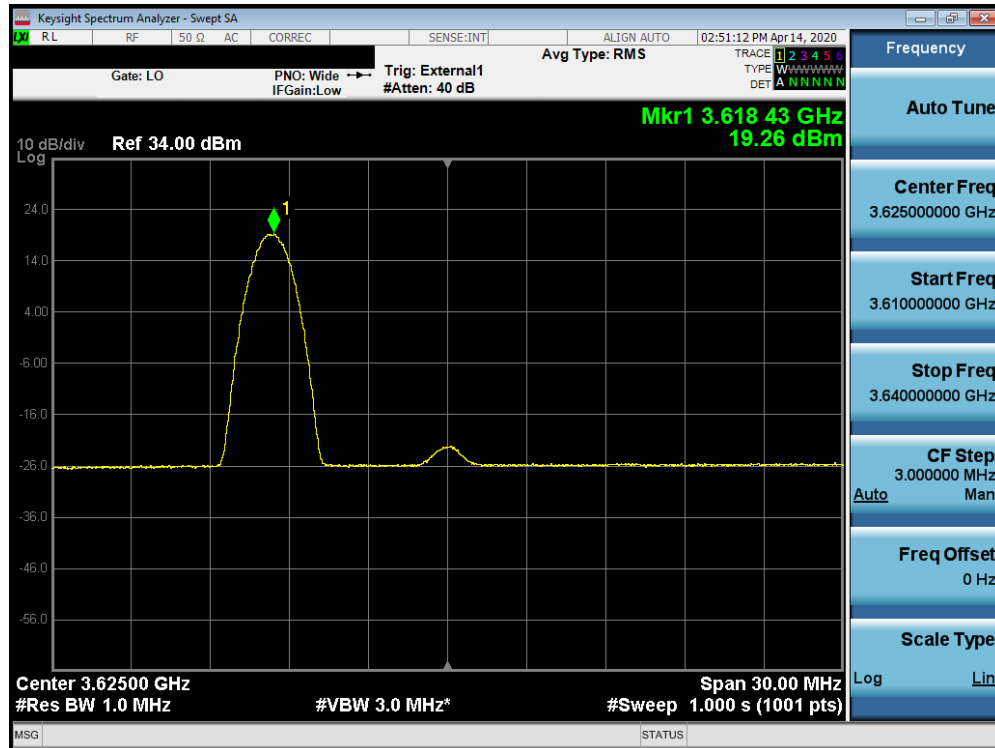
Plot 7-80. Peak Power Spectral Density Plot (B48 – 15.0MHz 16-QAM – Mid Channel RB: 1 RB, Offset: 0)
