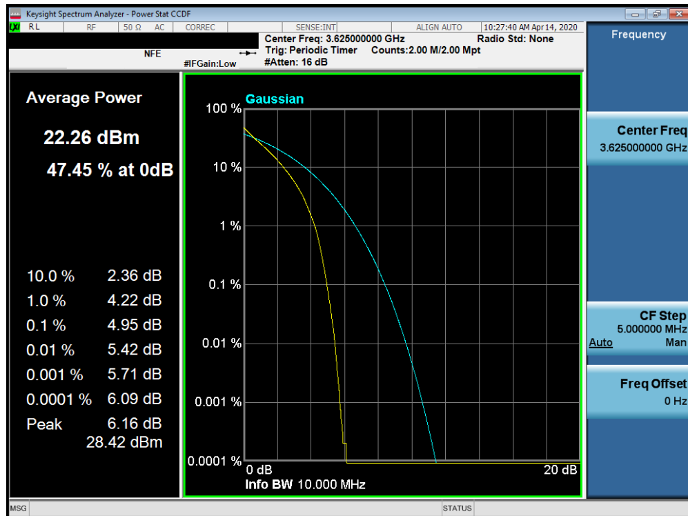
Plot 7-97. PAR Plot (Band 48 – 10.0MHz QPSK – Full RB Configuration)
