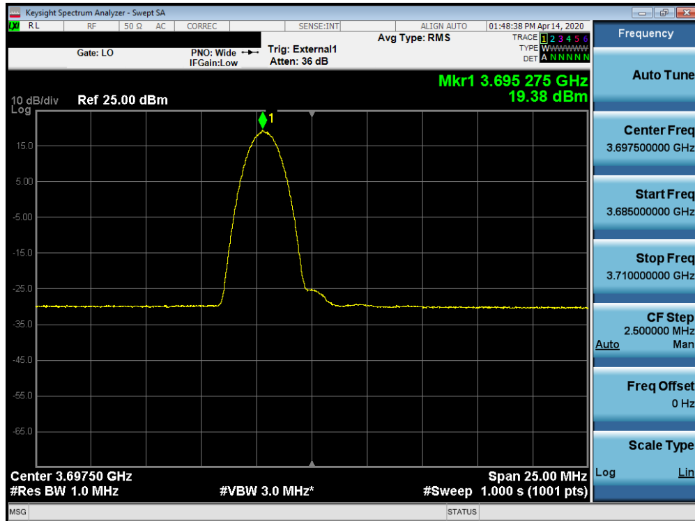
Plot 7-66. Peak Power Spectral Density Plot (B48 – 5.0MHz 64-QAM – High Channel RB: 1 RB, Offset: 0)
