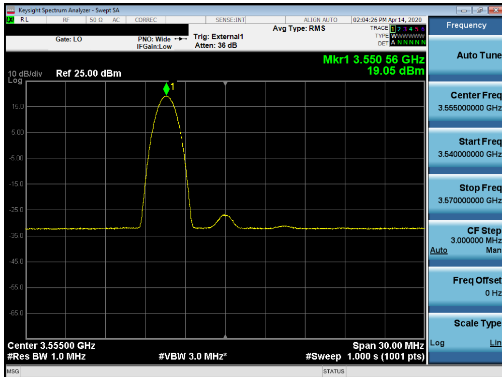
Plot 7-67. Peak Power Spectral Density Plot (B48 – 10.0MHz QPSK – Low Channel RB: 1 RB, Offset: 0)
