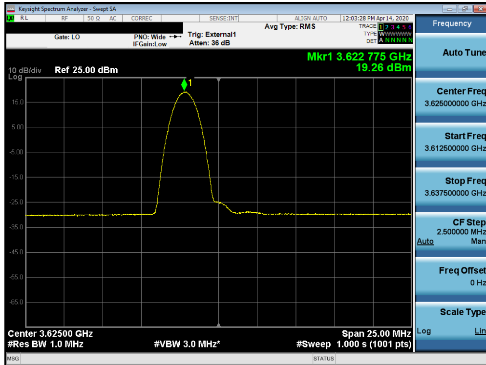
Plot 7-62. Peak Power Spectral Density Plot (B48 – 5.0MHz 16-QAM – Mid Channel RB: 1 RB, Offset: 0)
