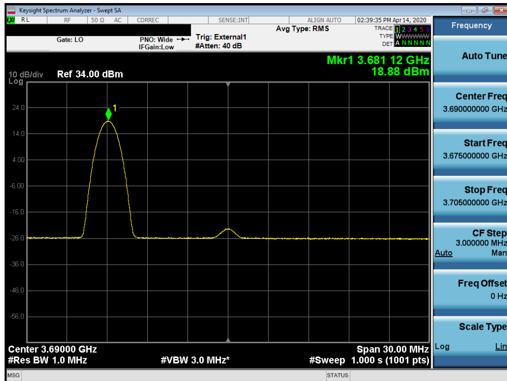
Plot 7-91. Peak Power Spectral Density Plot (B48 – 20.0MHz QPSK – High Channel RB: 1 RB, Offset: 0)
