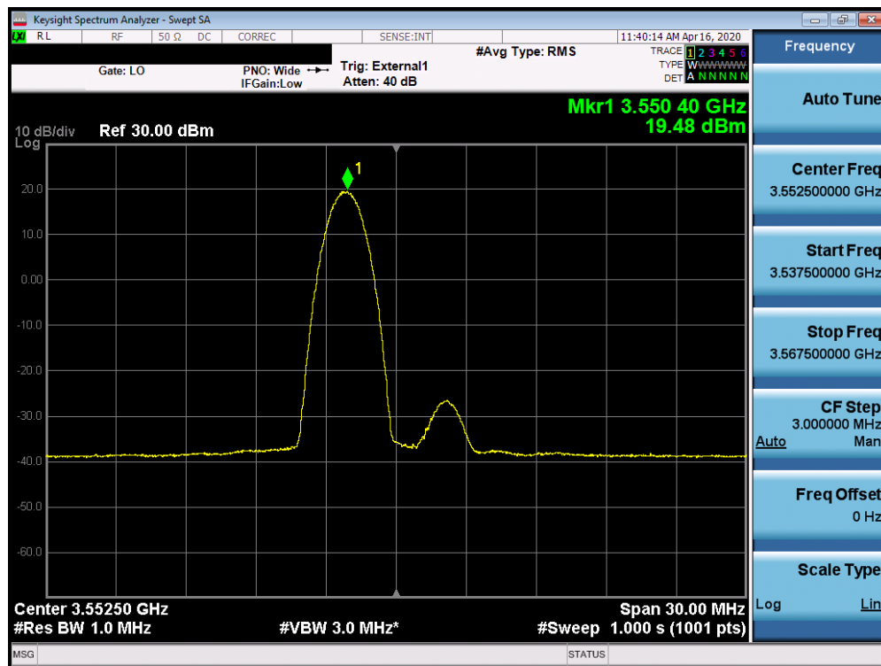
Plot 7-59. Peak Power Spectral Density Plot (B48 – 5.0MHz 16-QAM – Low Channel RB: 1 RB, Offset: 0)
