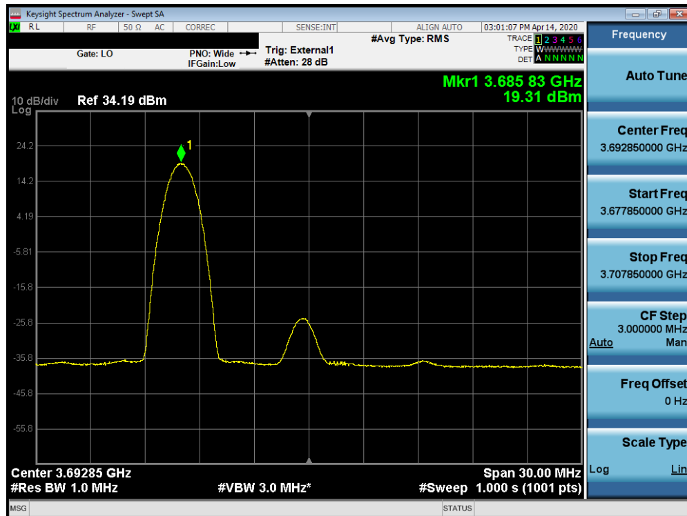
Plot 7-83. Peak Power Spectral Density Plot (B48 – 15.0MHz 16-QAM – High Channel RB: 1 RB, Offset: 0)
