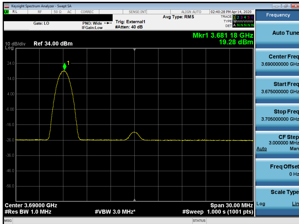
Plot 7-93. Peak Power Spectral Density Plot (B48 – 20.0MHz 64-QAM – High Channel RB: 1 RB, Offset: 0)
