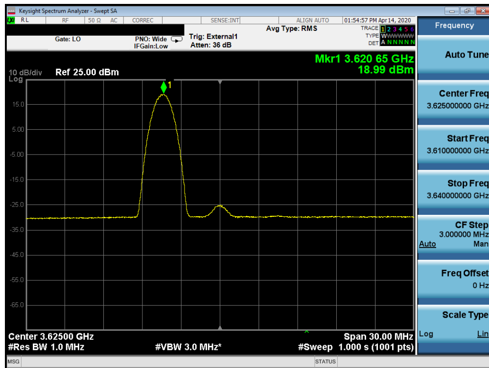
Plot 7-71. Peak Power Spectral Density Plot (B48 – 10.0MHz 16-QAM – Mid Channel RB: 1 RB, Offset: 0)
