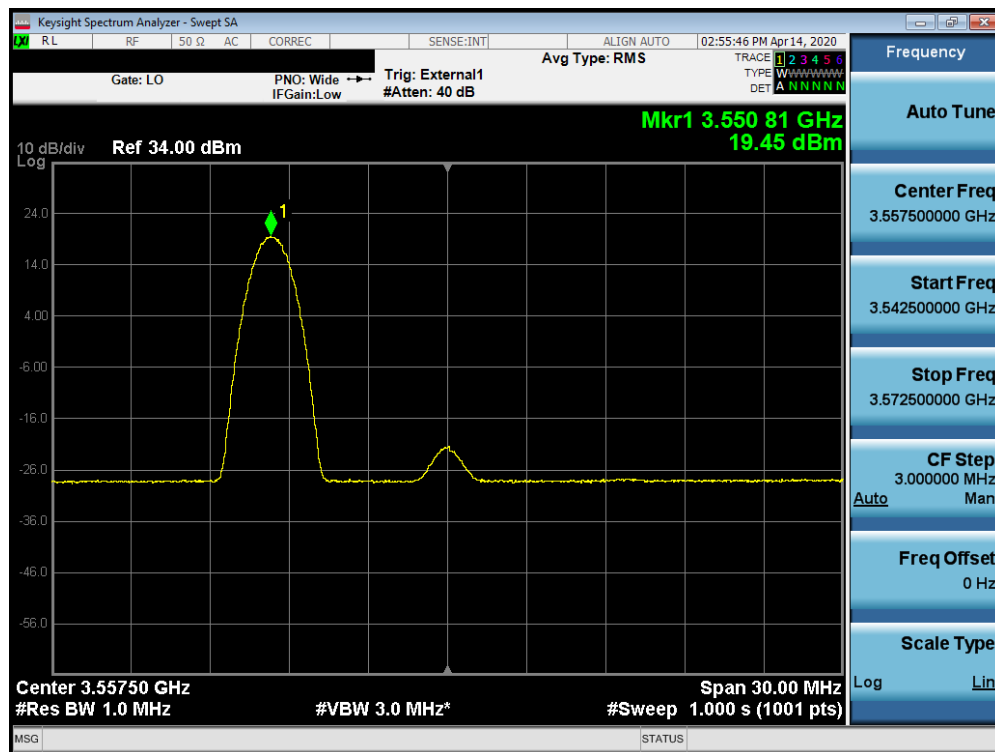
Plot 7-77. Peak Power Spectral Density Plot (B48 – 15.0MHz 16-QAM – Low Channel RB: 1 RB, Offset: 0)
