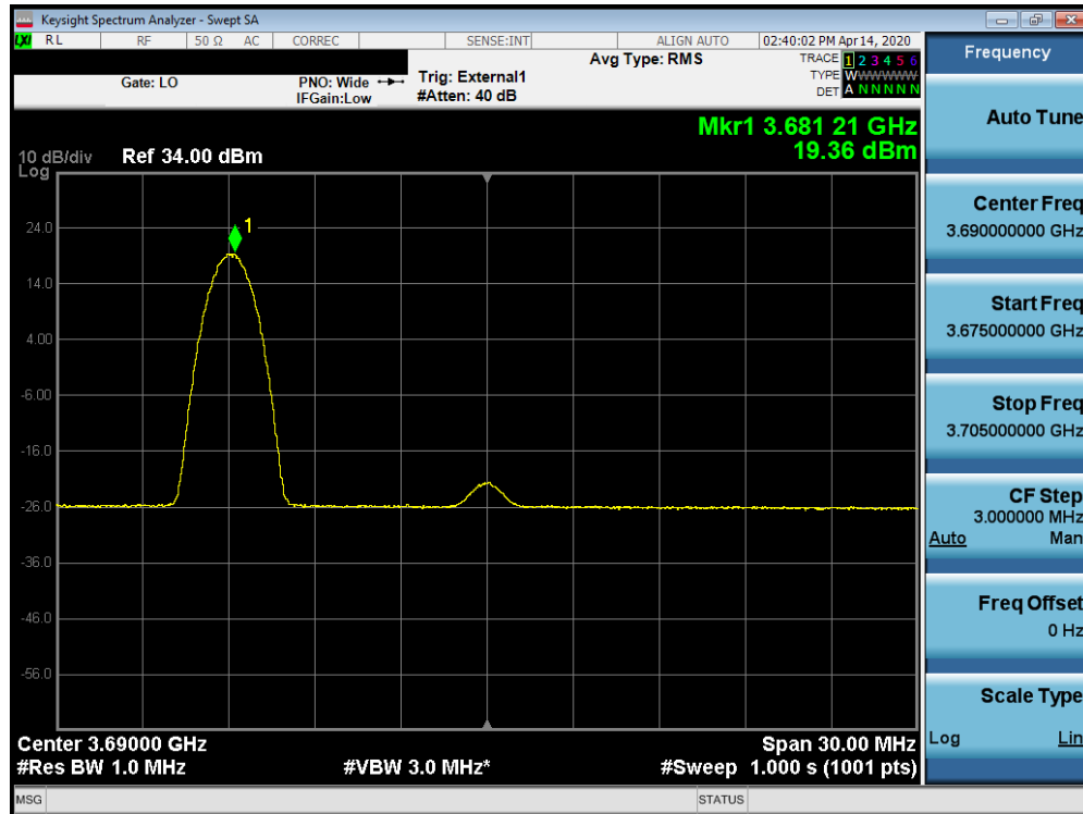
Plot 7-92. Peak Power Spectral Density Plot (B48 – 20.0MHz 16-QAM – High Channel RB: 1 RB, Offset: 0)
