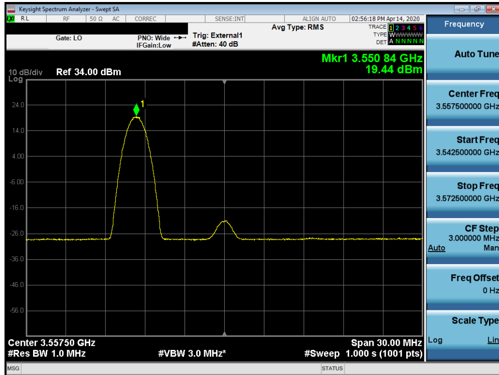
Plot 7-78. Peak Power Spectral Density Plot (B48 – 15.0MHz 64-QAM – Low Channel RB: 1 RB, Offset: 0)
