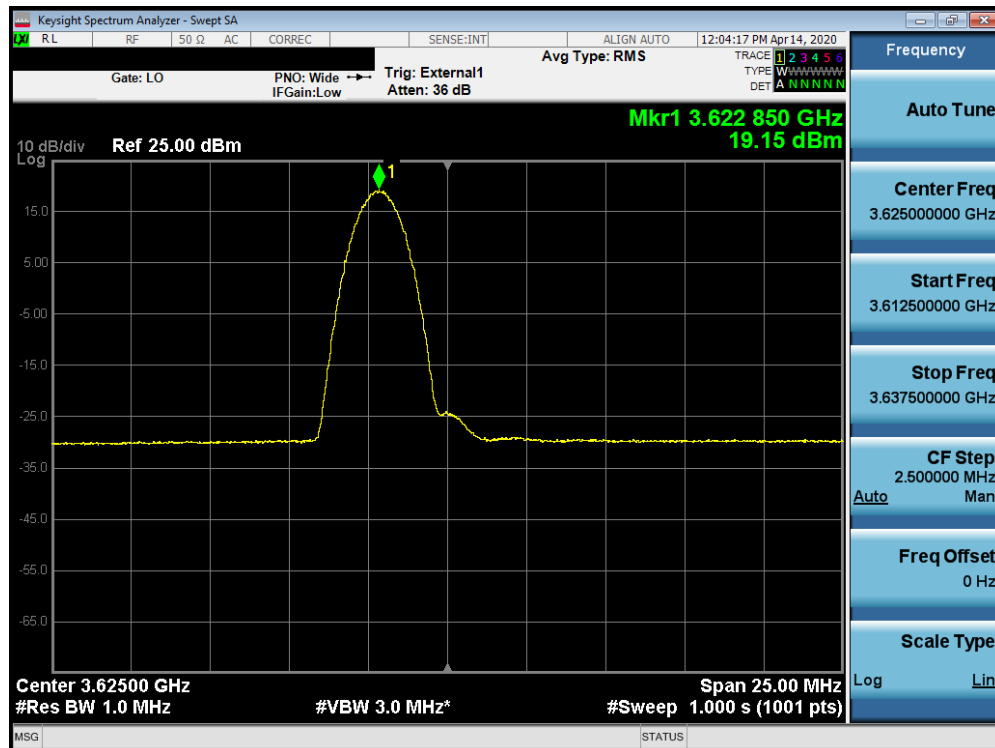
Plot 7-63. Peak Power Spectral Density Plot (B48 – 5.0MHz 64-QAM – Mid Channel RB: 1 RB, Offset: 0)
