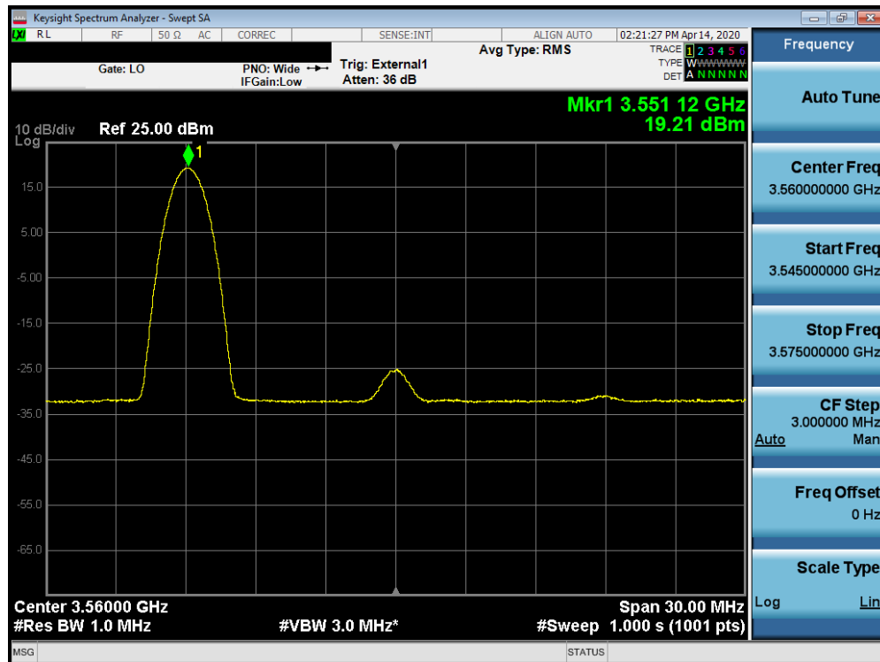
Plot 7-85. Peak Power Spectral Density Plot (B48 – 20.0MHz QPSK – Low Channel RB: 1 RB, Offset: 0)
