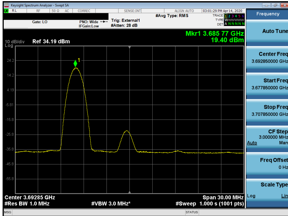
Plot 7-84. Peak Power Spectral Density Plot (B48 – 15.0MHz 64-QAM – High Channel RB: 1 RB, Offset: 0)
