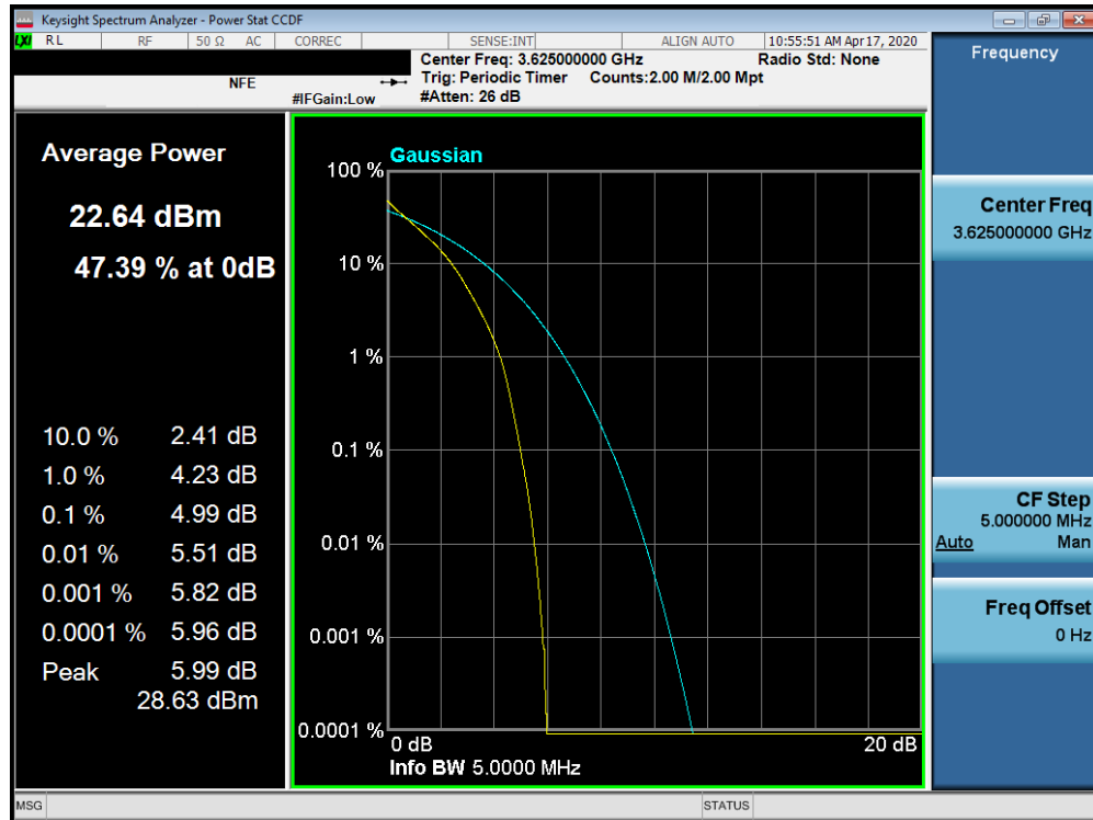
Plot 7-94. PAR Plot (Band 48 – 5.0MHz QPSK – Full RB Configuration)
