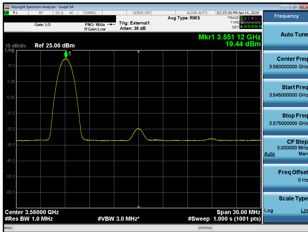
Plot 7-86. Peak Power Spectral Density Plot (B48 – 20.0MHz 16-QAM – Low Channel RB: 1 RB, Offset: 0)
