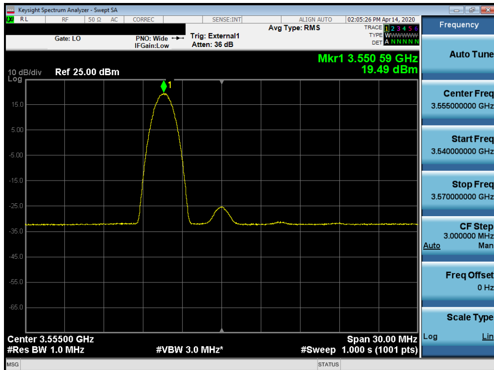
Plot 7-69. Peak Power Spectral Density Plot (B48 – 10.0MHz 64-QAM – Low Channel RB: 1 RB, Offset: 0)
