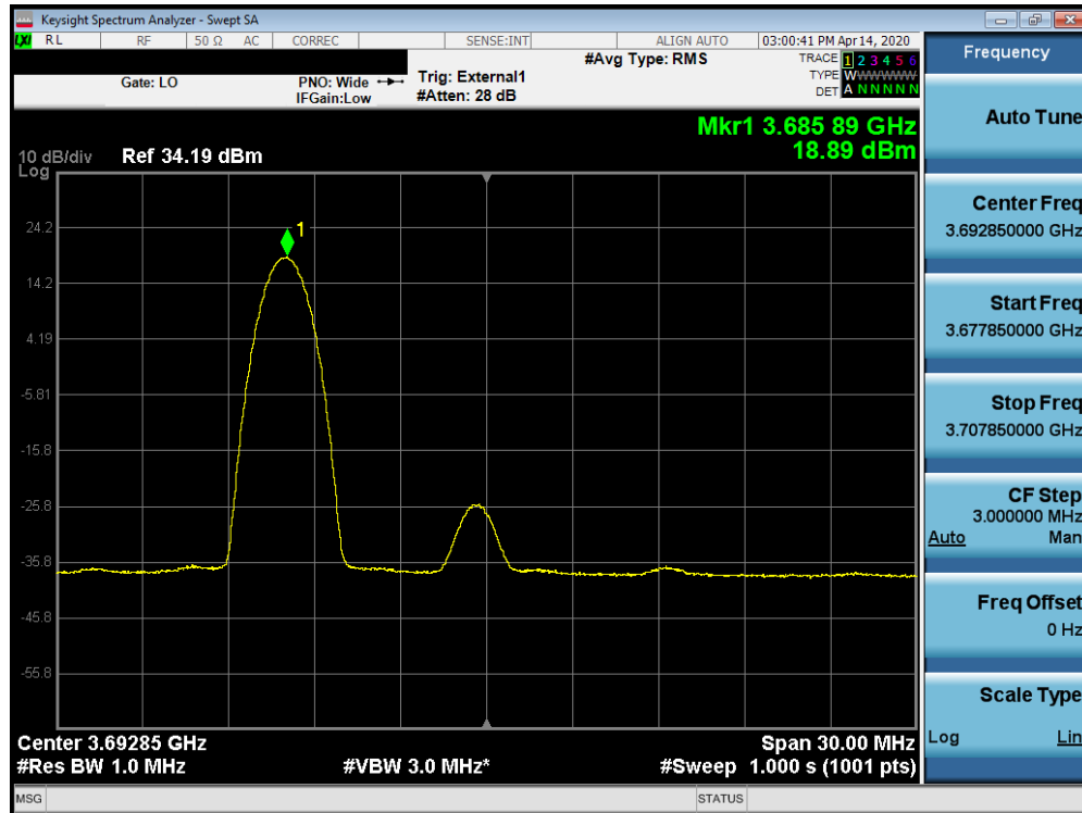
Plot 7-82. Peak Power Spectral Density Plot (B48 – 15.0MHz QPSK – High Channel RB: 1 RB, Offset: 0)
