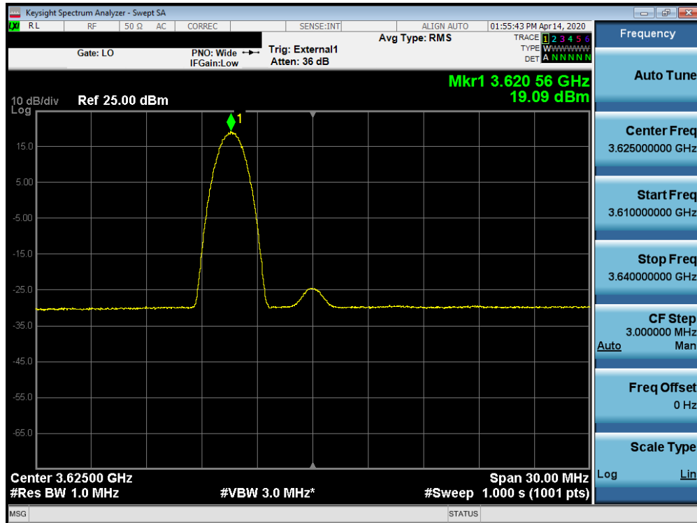
Plot 7-72. Peak Power Spectral Density Plot (B48 – 10.0MHz 64-QAM – Mid Channel RB: 1 RB, Offset: 0)
