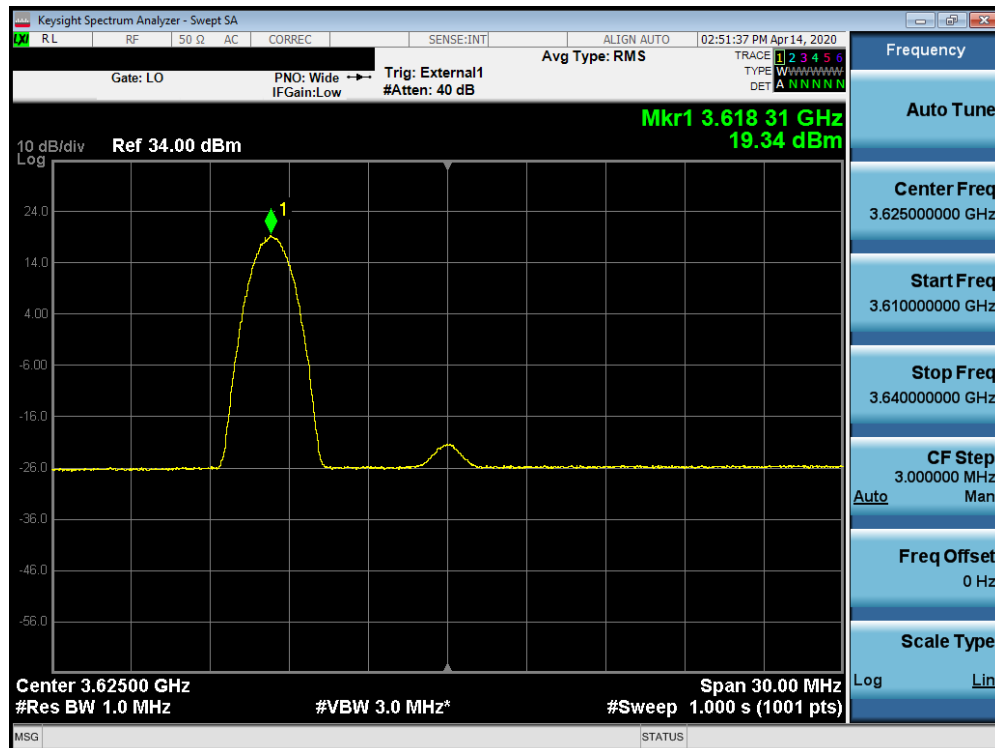
Plot 7-81. Peak Power Spectral Density Plot (B48 – 15.0MHz 64-QAM – Mid Channel RB: 1 RB, Offset: 0)
