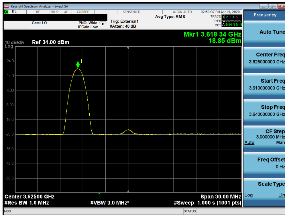
Plot 7-79. Peak Power Spectral Density Plot (B48 – 15.0MHz QPSK – Mid Channel RB: 1 RB, Offset: 0)
