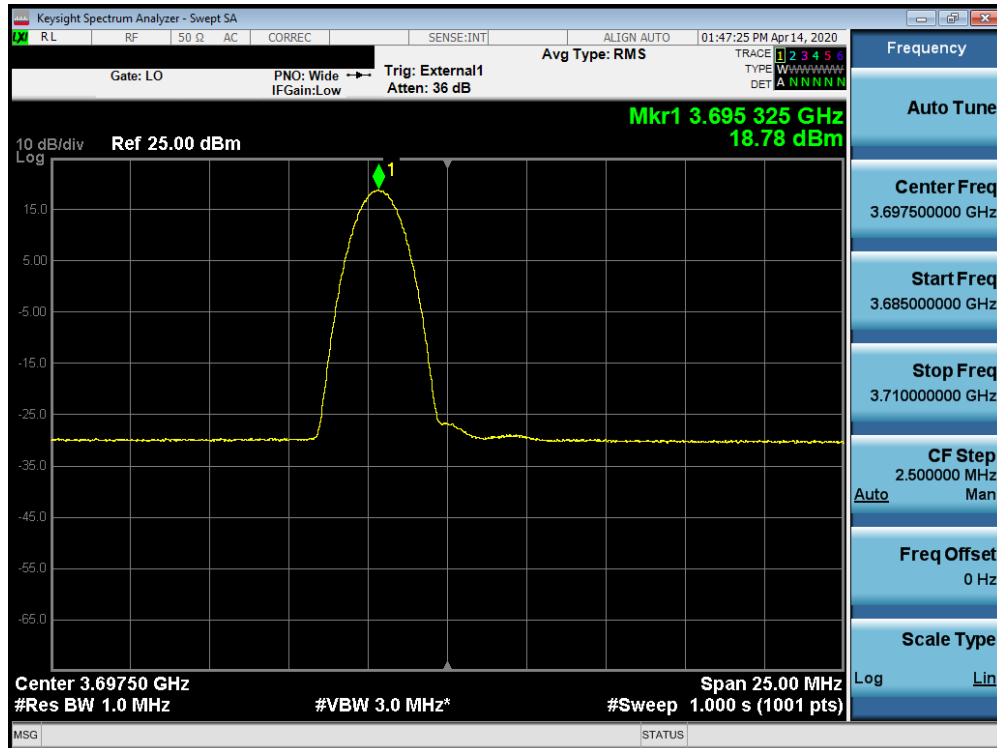
Plot 7-64. Peak Power Spectral Density Plot (B48 – 5.0MHz QPSK – High Channel RB: 1 RB, Offset: 0)
