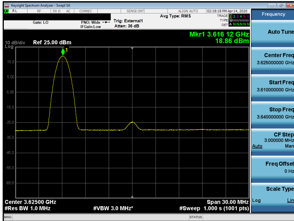
Plot 7-88. Peak Power Spectral Density Plot (B48 – 20.0MHz QPSK – Mid Channel RB: 1 RB, Offset: 0)
