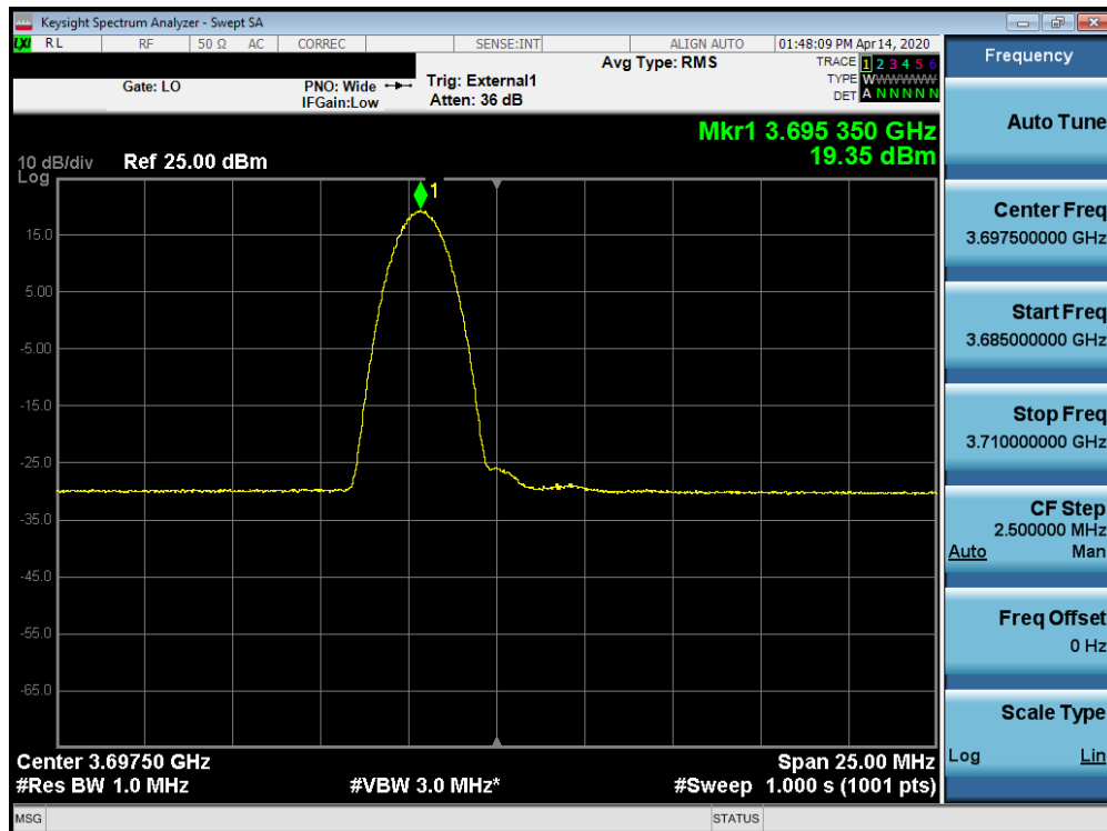
Plot 7-65. Peak Power Spectral Density Plot (B48 – 5.0MHz 16-QAM – High Channel RB: 1 RB, Offset: 0)
