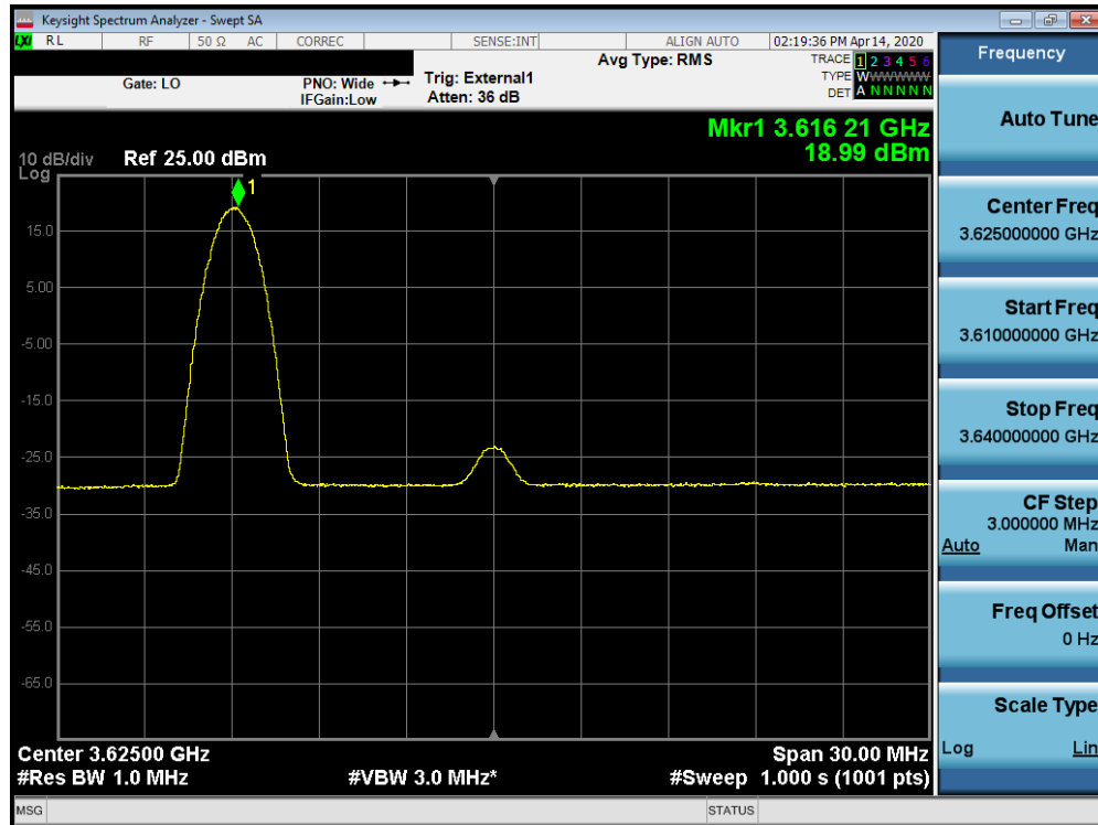
Plot 7-90. Peak Power Spectral Density Plot (B48 – 20.0MHz 64-QAM – Mid Channel RB: 1 RB, Offset: 0)
