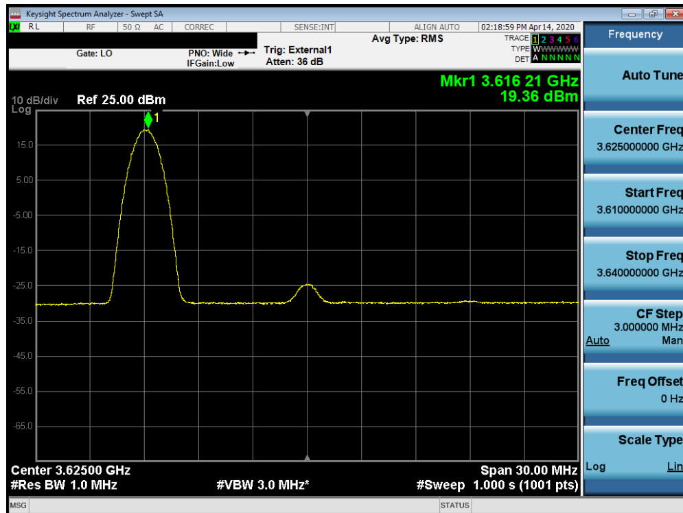
Plot 7-89. Peak Power Spectral Density Plot (B48 – 20.0MHz 16-QAM – Mid Channel RB: 1 RB, Offset: 0)
