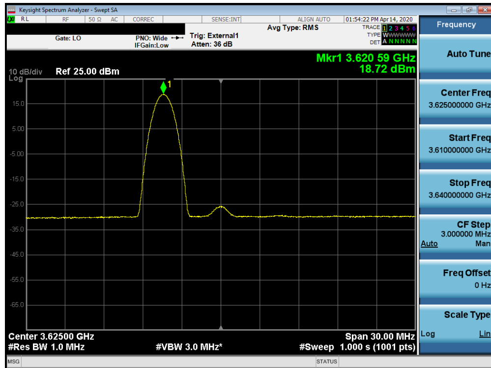
Plot 7-70. Peak Power Spectral Density Plot (B48 – 10.0MHz QPSK – Mid Channel RB: 1 RB, Offset: 0)
