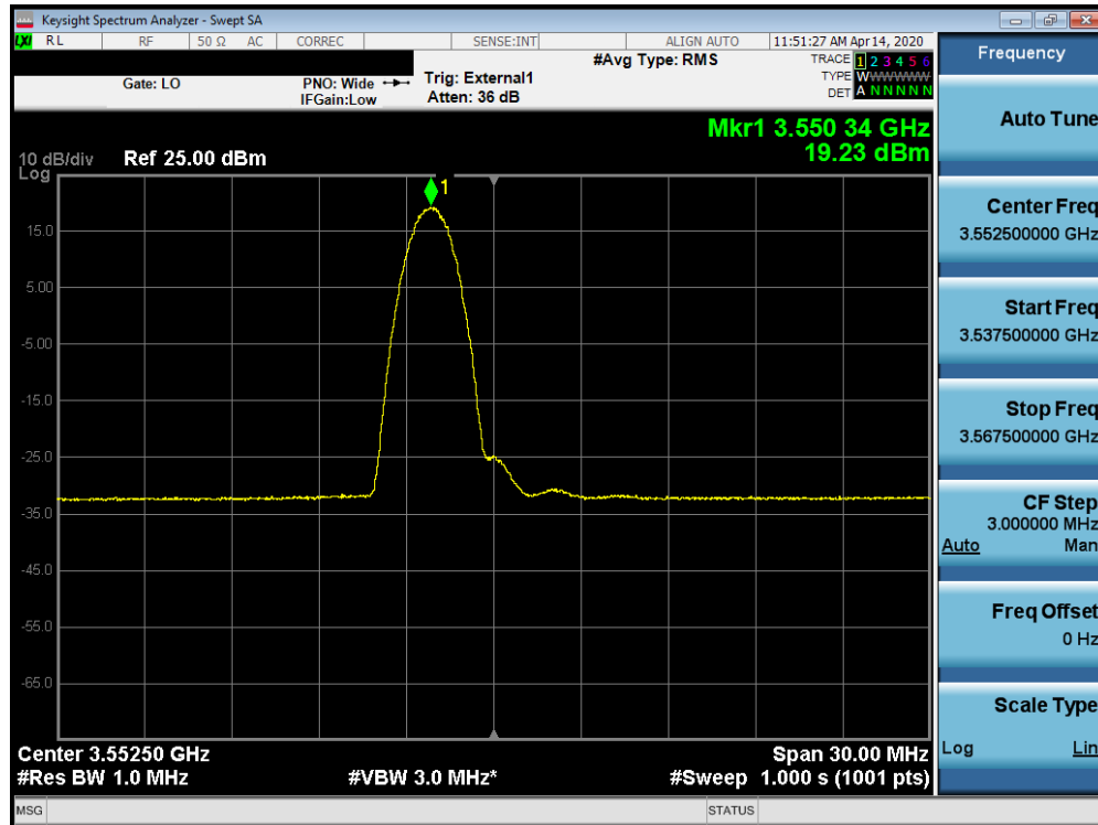
Plot 7-60. Peak Power Spectral Density Plot (B48 – 5.0MHz 64-QAM – Low Channel RB: 1 RB, Offset: 0)
