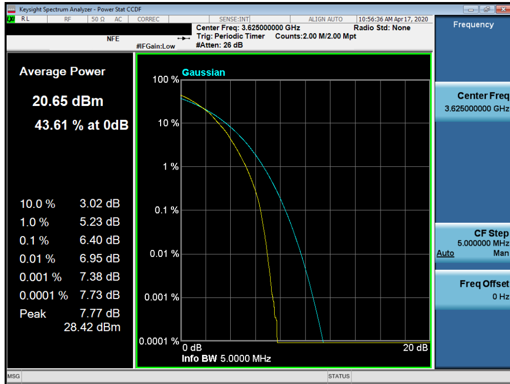
Plot 7-96. PAR Plot (Band 48 – 5.0MHz 64-QAM – Full RB Configuration)
