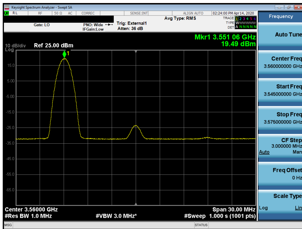
Plot 7-87. Peak Power Spectral Density Plot (B48 – 20.0MHz 64-QAM – Low Channel RB: 1 RB, Offset: 0)
