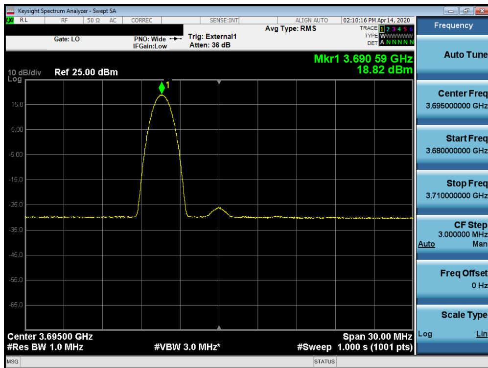
Plot 7-73. Peak Power Spectral Density Plot (B48 – 10.0MHz QPSK – High Channel RB: 1 RB, Offset: 0)
