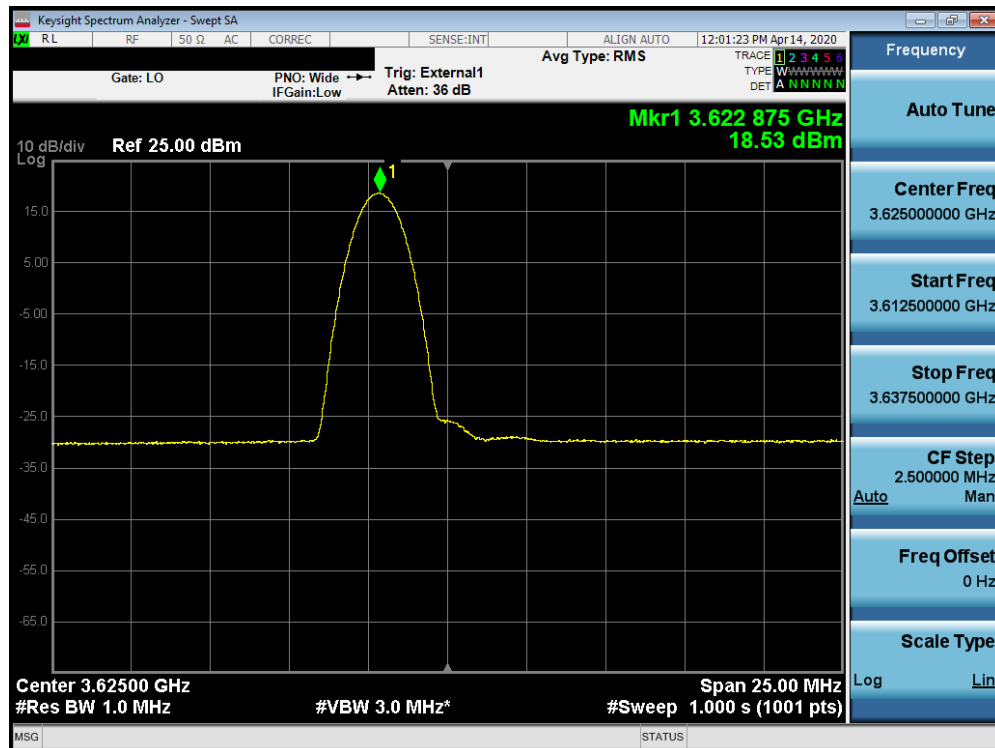
Plot 7-61. Peak Power Spectral Density Plot (B48 – 5.0MHz QPSK – Mid Channel RB: 1 RB, Offset: 0)
