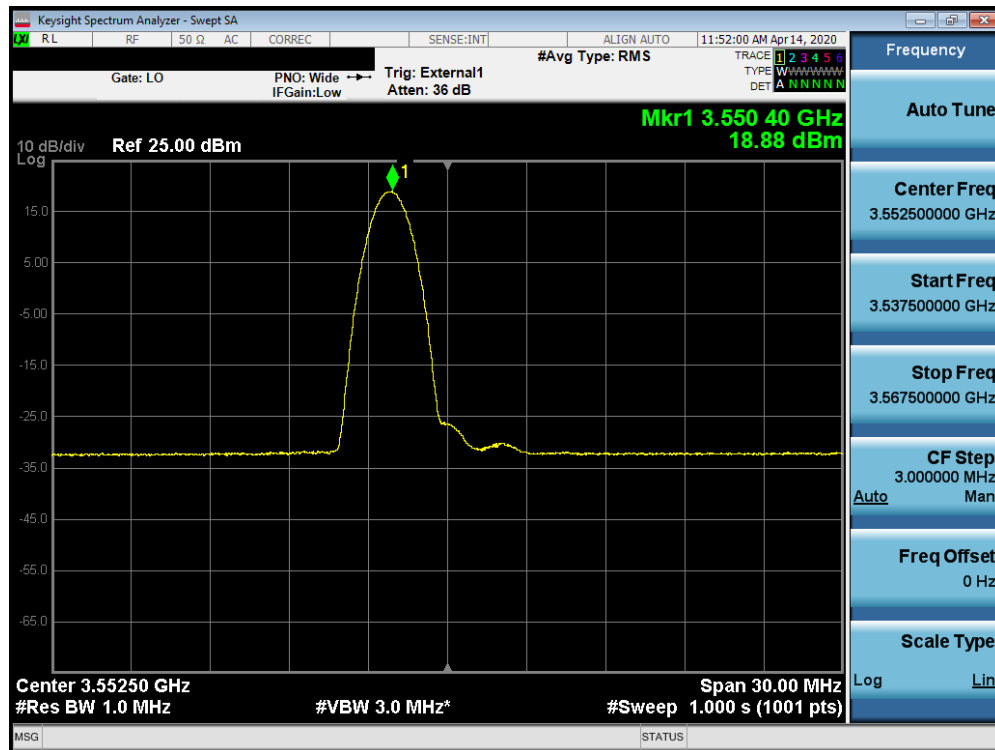
Plot 7-58. Peak Power Spectral Density Plot (B48 – 5.0MHz QPSK – Low Channel RB: 1 RB, Offset: 0)
