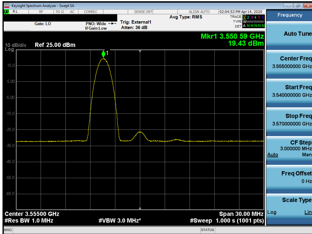
Plot 7-68. Peak Power Spectral Density Plot (B48 – 10.0MHz 16-QAM – Low Channel RB: 1 RB, Offset: 0)
