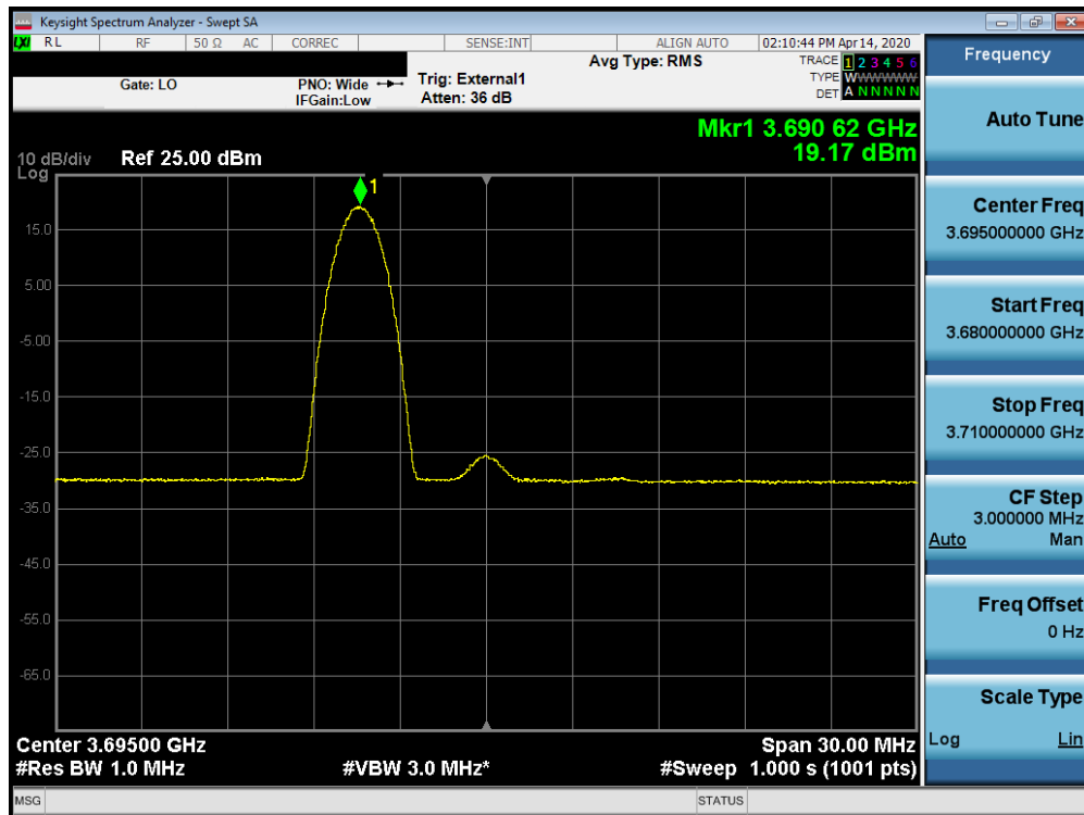
Plot 7-74. Peak Power Spectral Density Plot (B48 – 10.0MHz 16-QAM – High Channel RB: 1 RB, Offset: 0)
