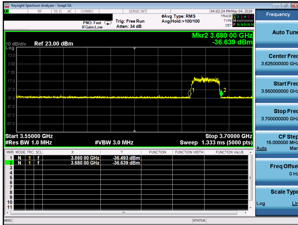
Plot 16. Conducted Measurement – UUT RF transmission range and bandwidths are less or equal to frequency range and bandwidth of compatible BTS-CBSD (WINNF.T.C.HBT.7)
