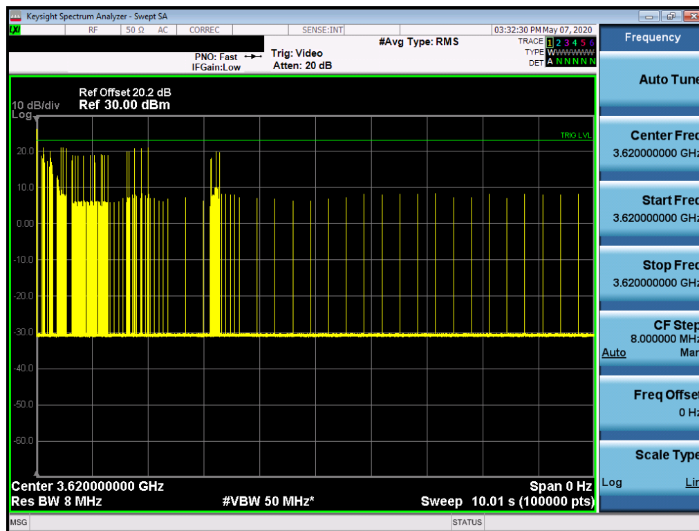
Plot 34. 10s Time Domain Sweep
