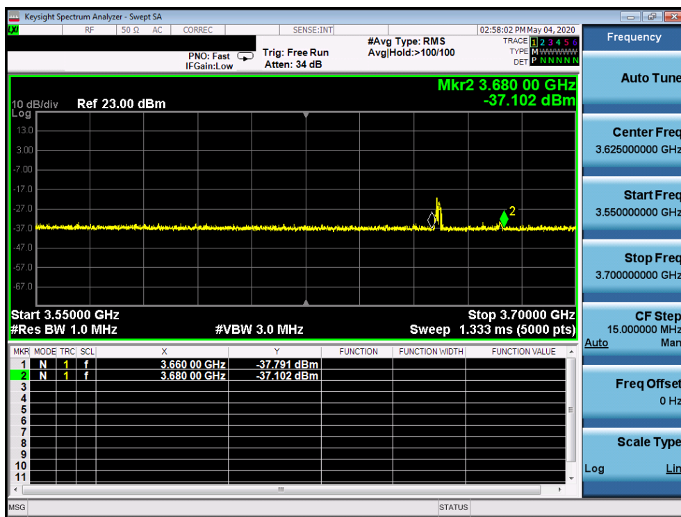
Plot 3. Conducted Measurement – UUT RF transmission range and bandwidths are less or equal to frequency range and bandwidth of compatible BTS-CBSD(WINNF.FT.C.REG.8)
