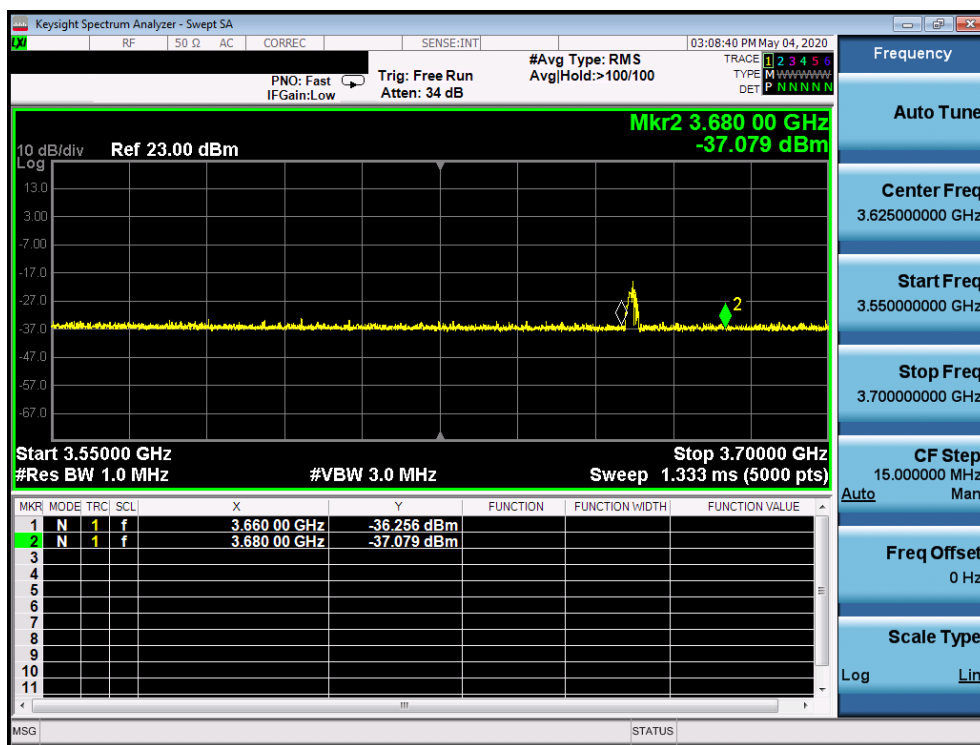
Plot 8. Conducted Measurement – UUT RF transmission range and bandwidths are less or equal to frequency range and bandwidth of compatible BTS-CBSD(WINNF.FT.C.REG.18)
