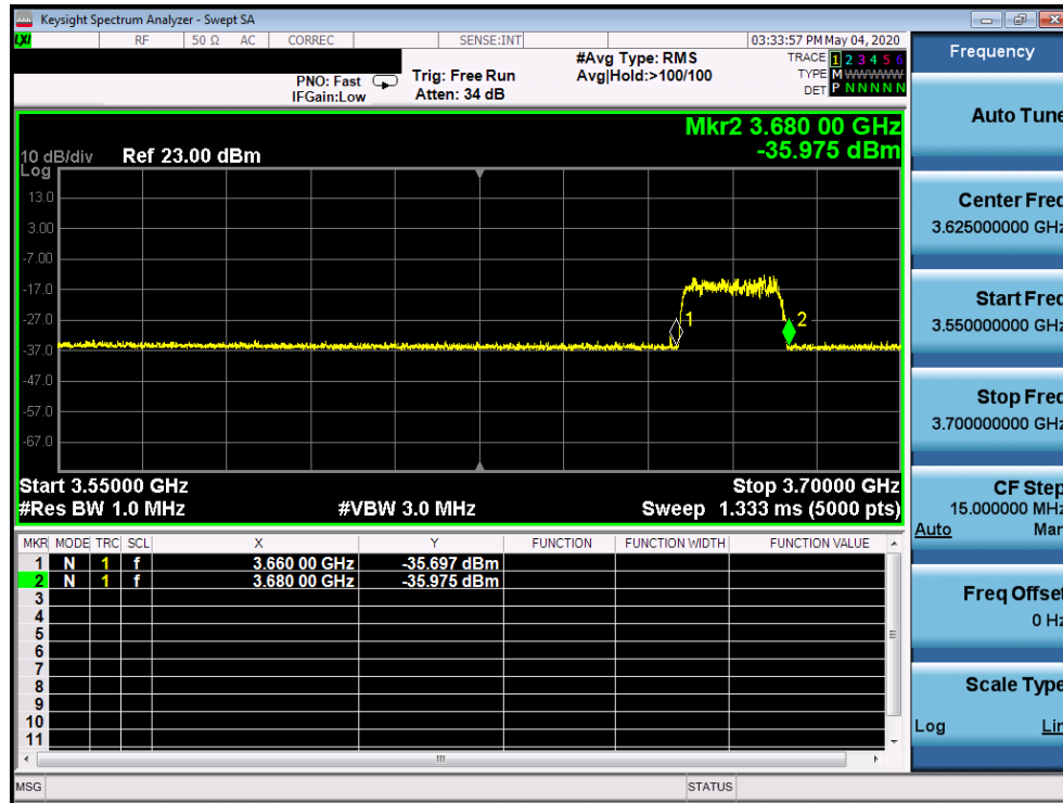
Plot 12. Conducted Measurement – UUT RF transmission range and bandwidths are less or equal to frequency range and bandwidth of compatible BTS-CBSD (WINNF.TT.C.HBT.3)
