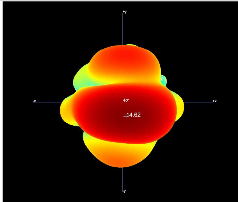
B1.5 3D Pattern for 2700MHz
