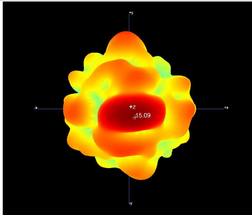
B1.3 3D Pattern for 4200MHz
