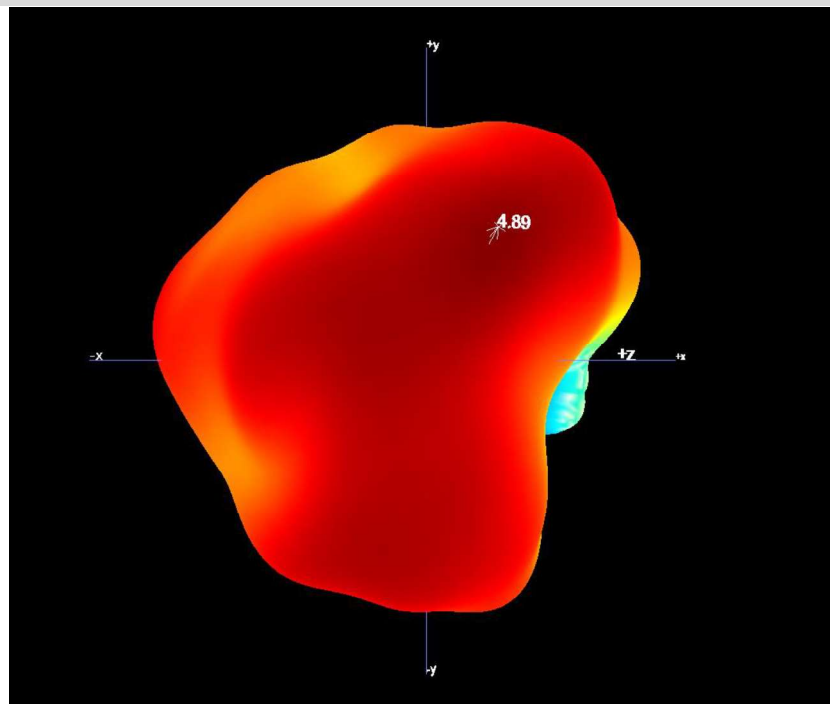
B1.16 3D Pattern for 1574.42MHz
