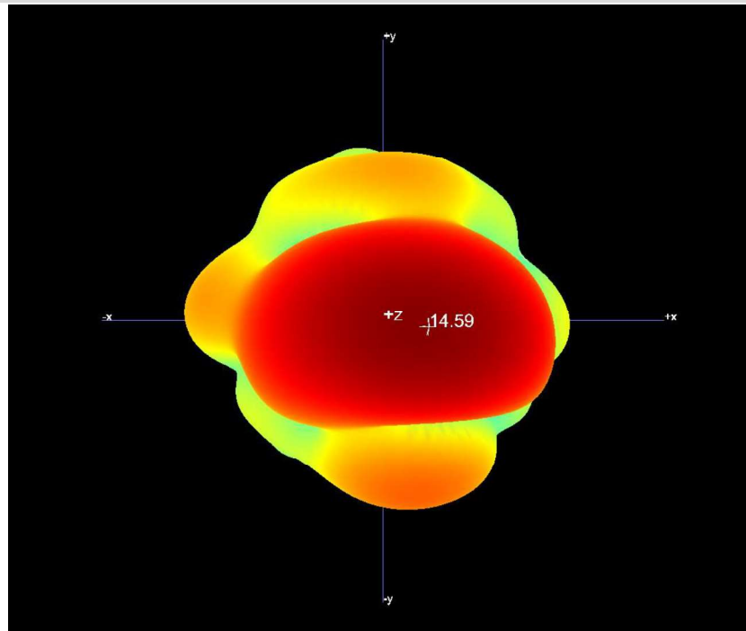
B1.2 3D Pattern for 2700MHz
