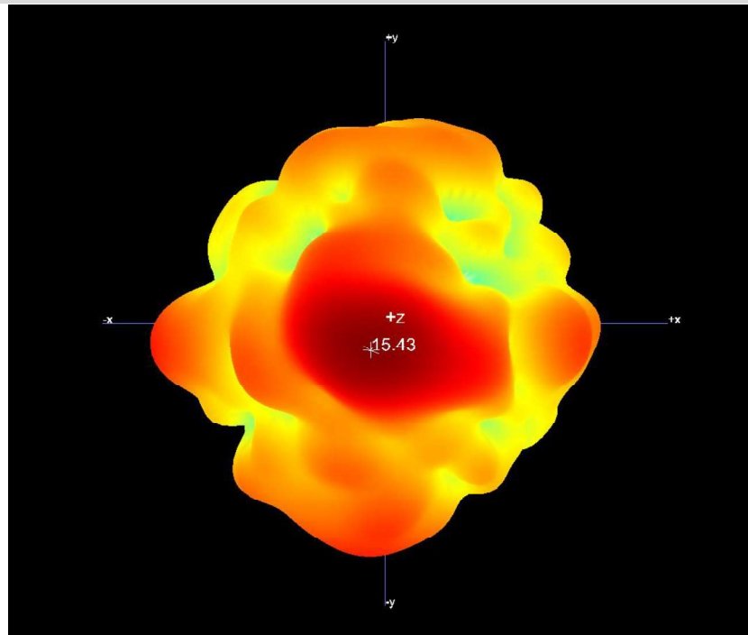
B1.6 3D Pattern for 4200MHz
