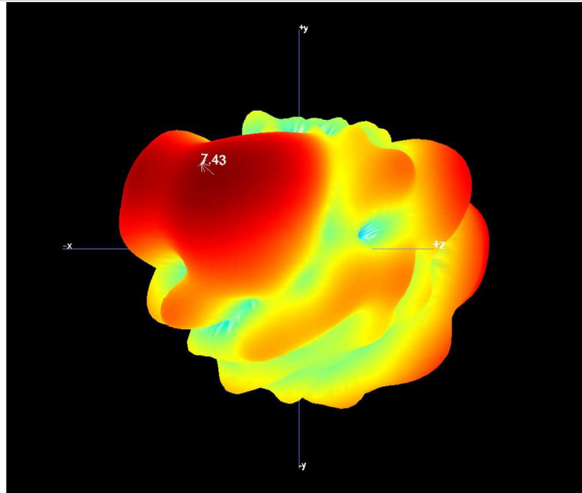
B1.15 3D Pattern for 2500MHz
