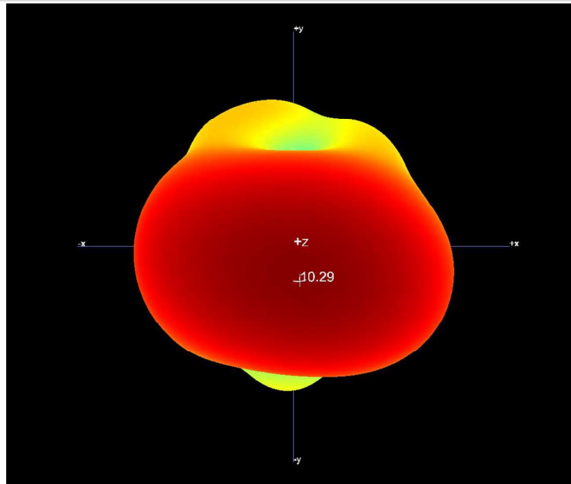
B1.1 3D Pattern for 1710MHz
