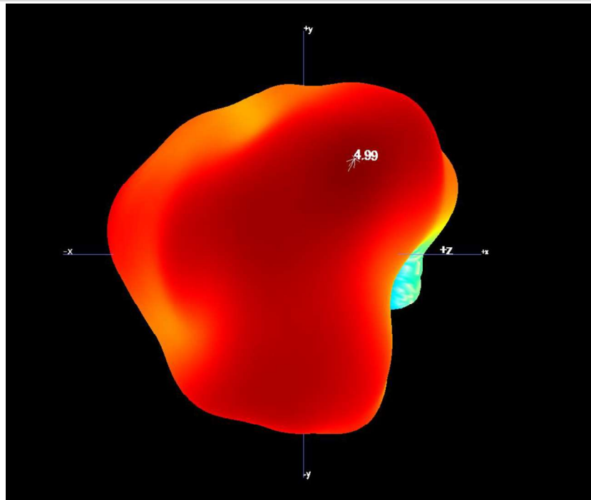
B1.18 3D Pattern for 1576.42MHz
