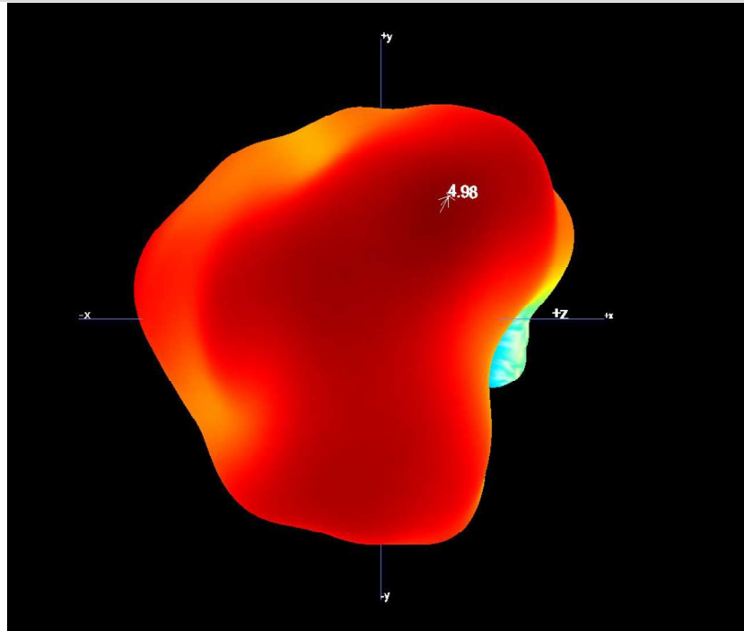
B1.17 3D Pattern for 1575.42MHz
