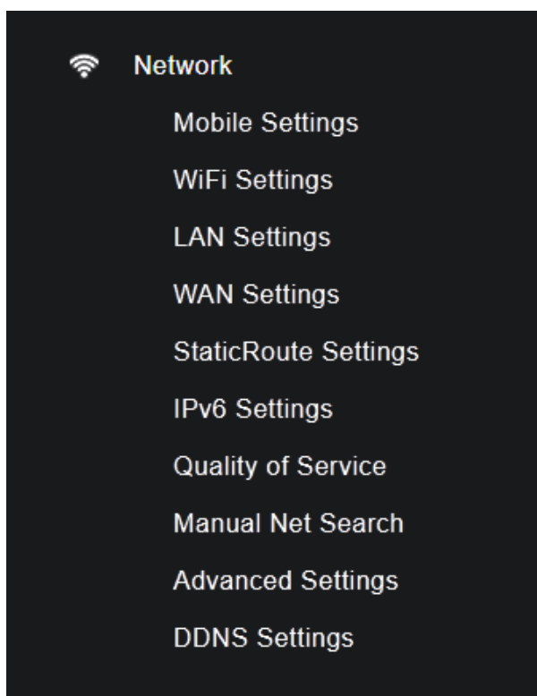
Figure 8 – Network menu
