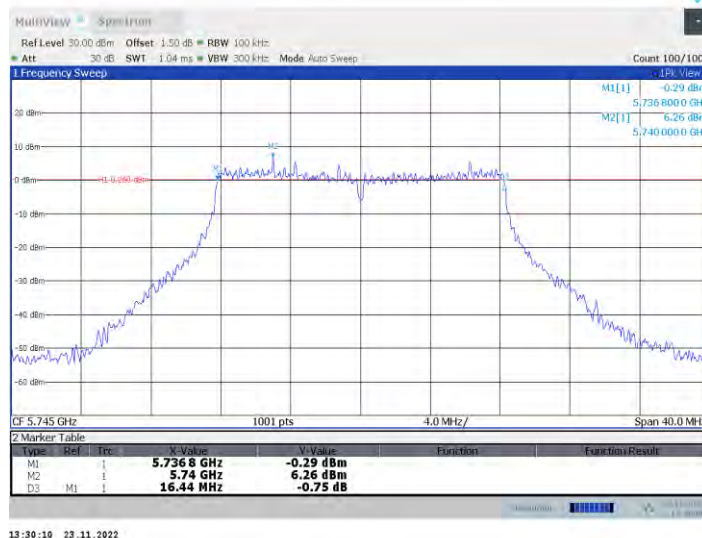
11a-CDD Ant4 5745
