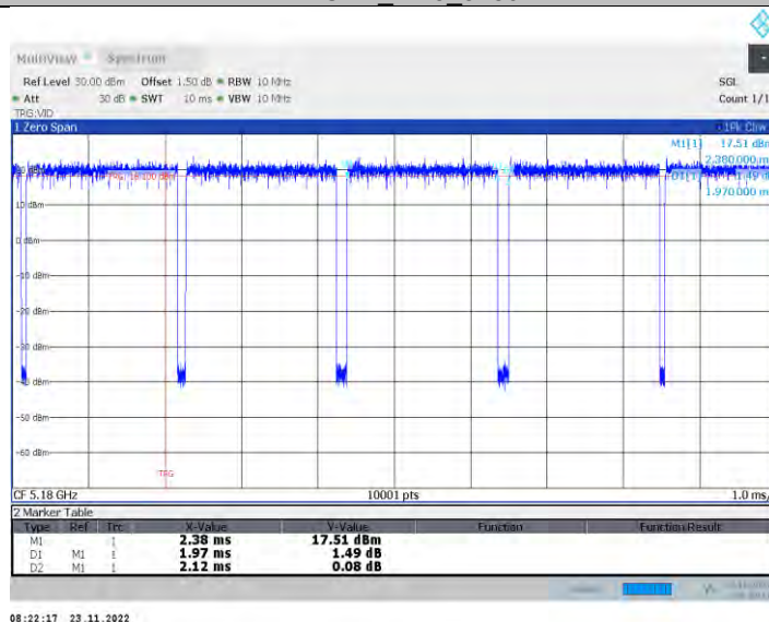
11a-CDD Ant4 5180
