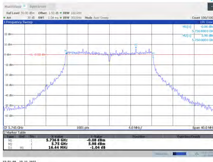
11a-CDD Ant4 5745
