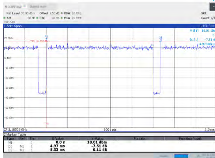
11ax20MIMO_Ant3_5180_26RU+26RU+26RU_Left
