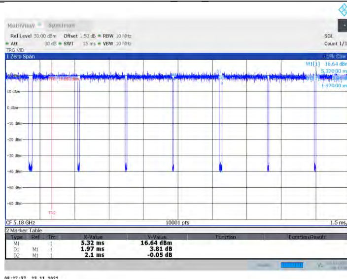
11a-CDD Ant4 5180
