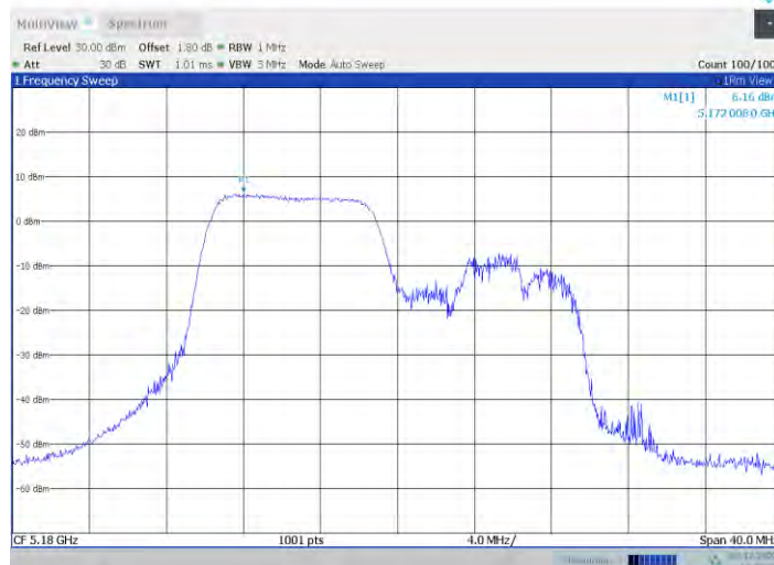
11ax20MIMO_Ant3_5180_26RU+26RU+26RU+26RU_Left
