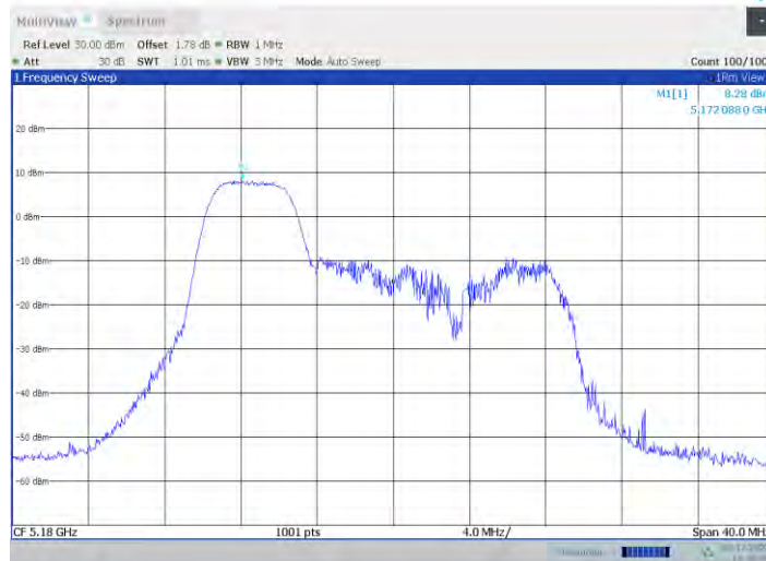
11ax20MIMO_Ant3_5180_26RU+26RU+26RU+26RU_Left
