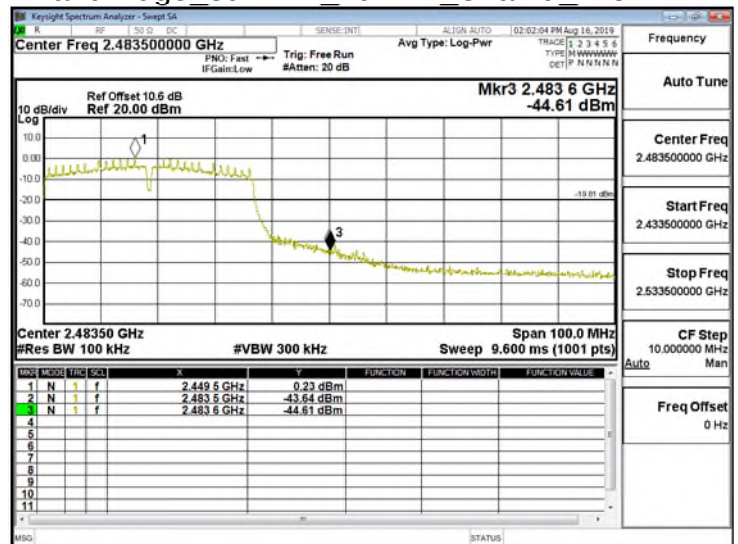
Band Edge_802.11n_40MHz_Chain0_2452MHz
