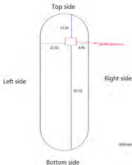
Fig.7 Antenna position of EUT
