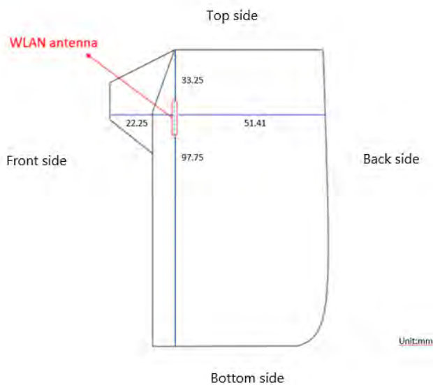
Fig.8 Antenna position of EUT
