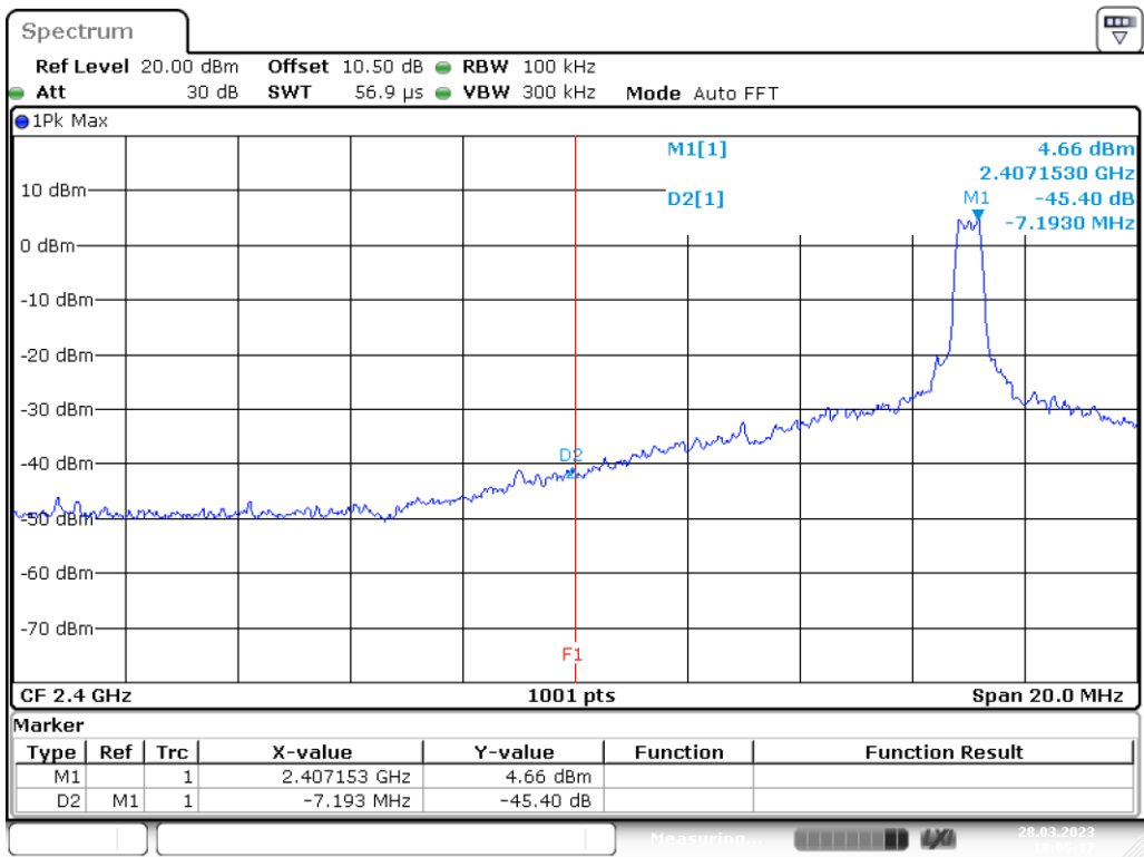
SRD Mode Band Edge, Left Side
