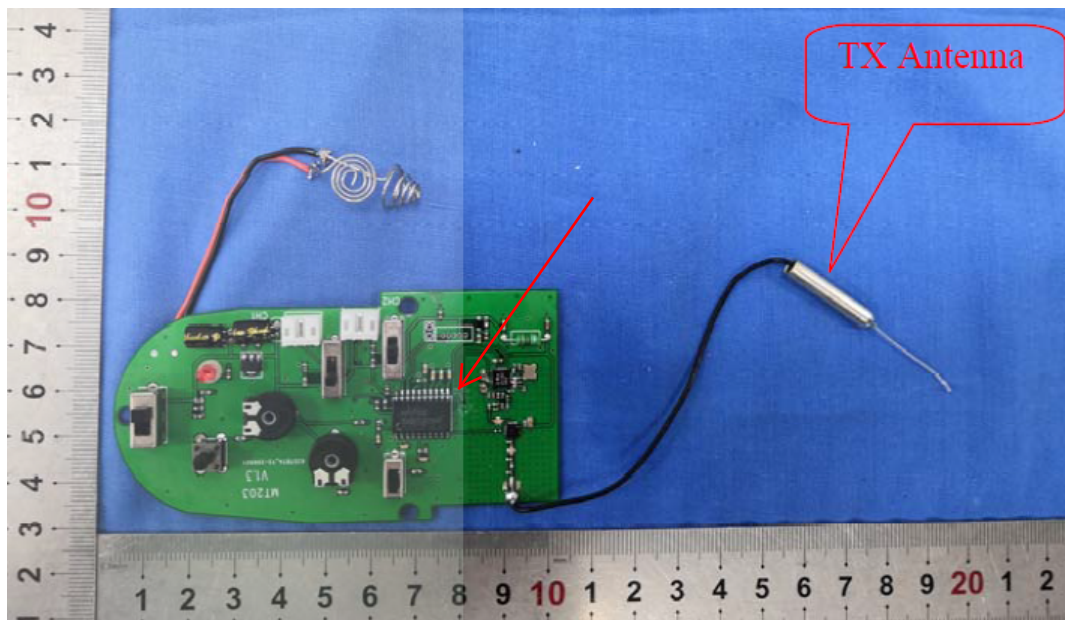
Original device
