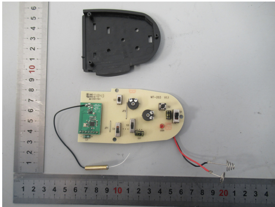
EUT – PCB Top View (MT-203)
