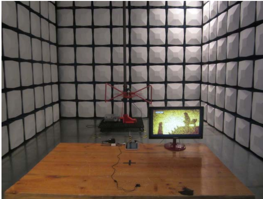
Radiated Emission Below 1GHz -Front View (HDMI)
