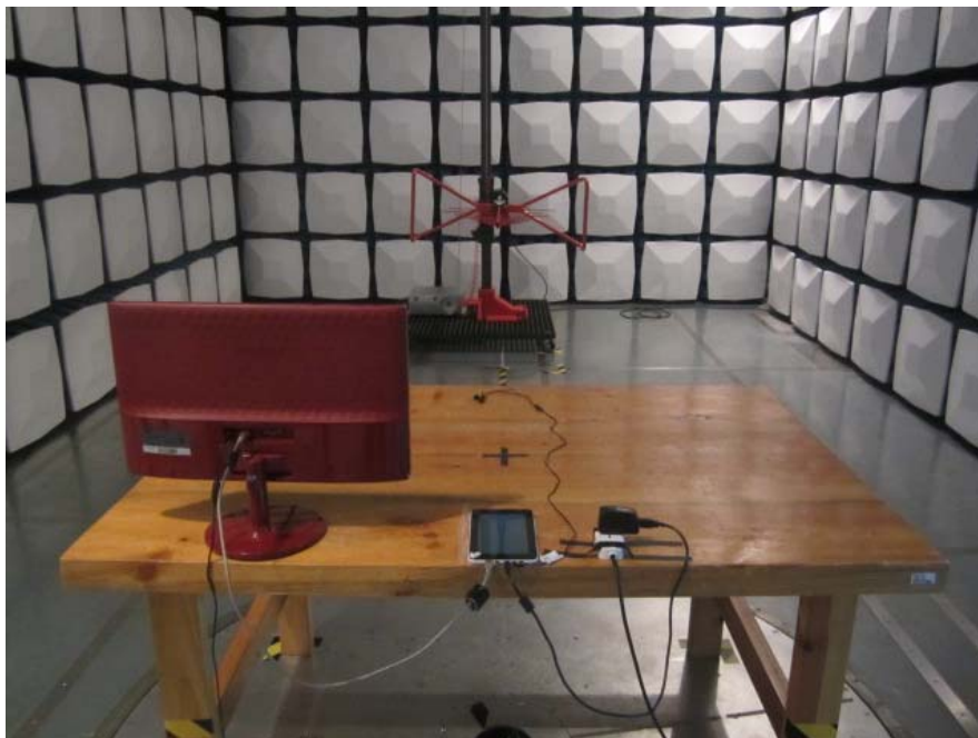
Radiated Emission Below 1GHz - Rear View (HDMI)
