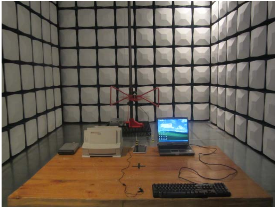
Radiated Emission Below 1GHz -Front View (Downloading)
