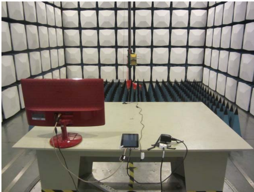
Radiated Emission Above 1GHz- Rear View (HDMI)
