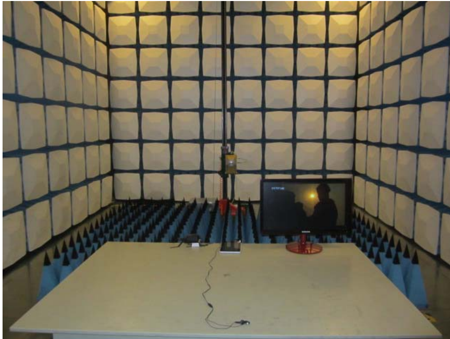
Radiated Emission Above 1GHz -Front View (HDMI)
