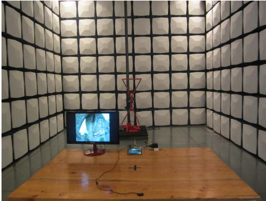
Radiated Emission Below 1GHz Front View (Charging&Playing Mode)
