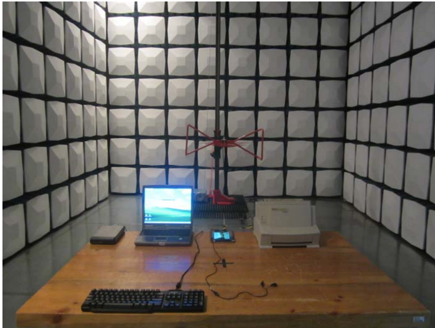
Radiated Emission Below 1GHz Front View (Downloading Mode)
