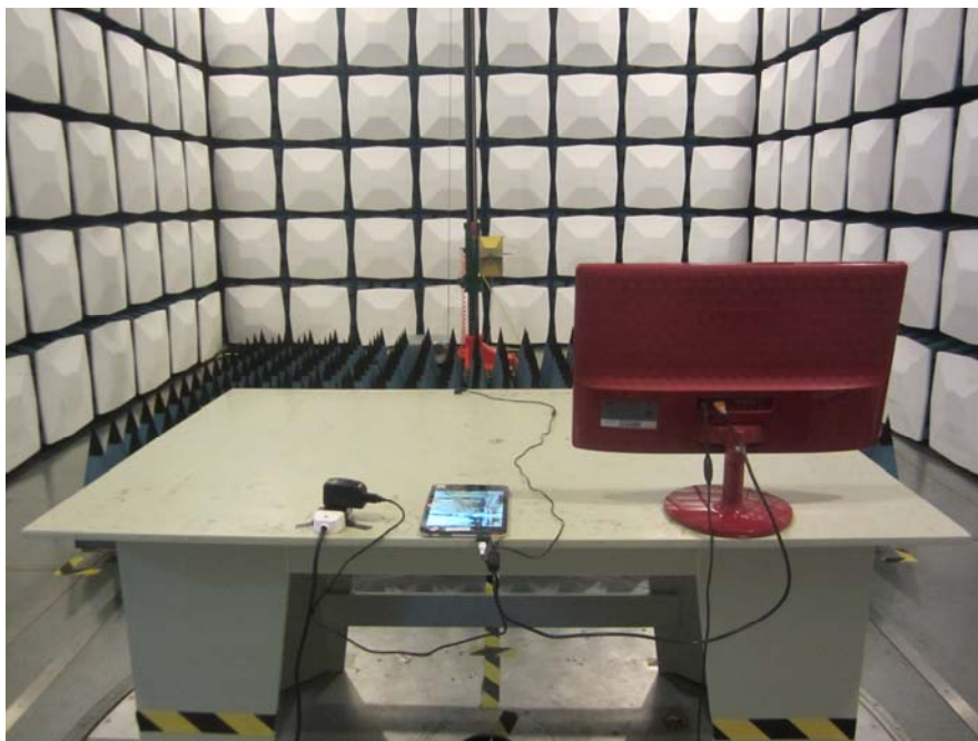
Radiated Emission Above 1GHz Rear View (Charging&Playing Mode)
