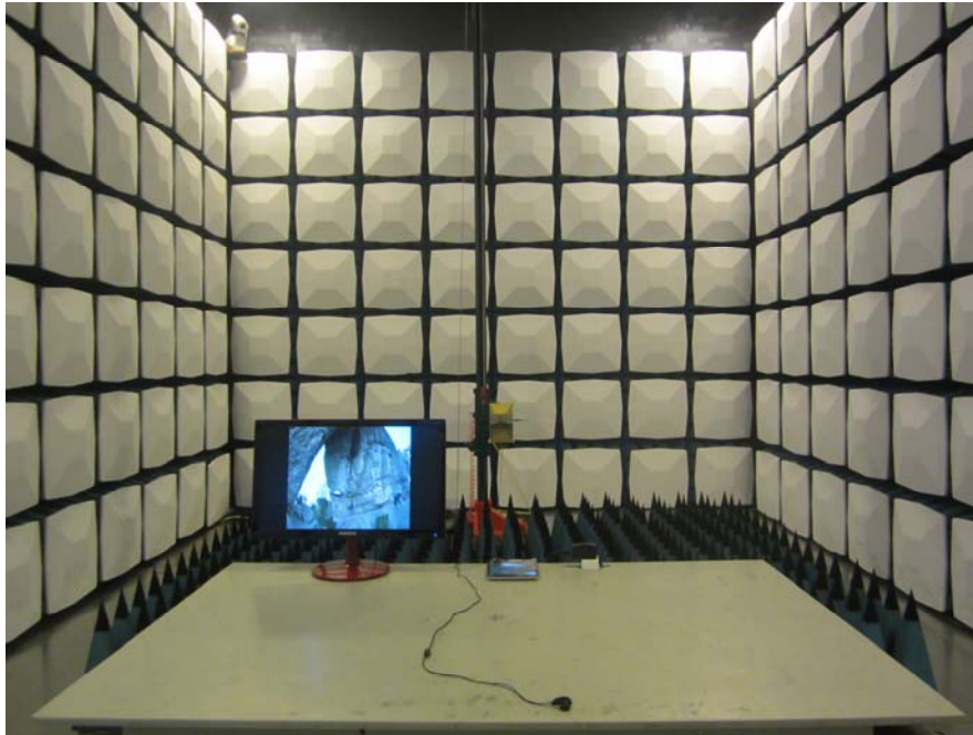
Radiated Emission Above 1GHz Front View (Charging&Playing Model)
