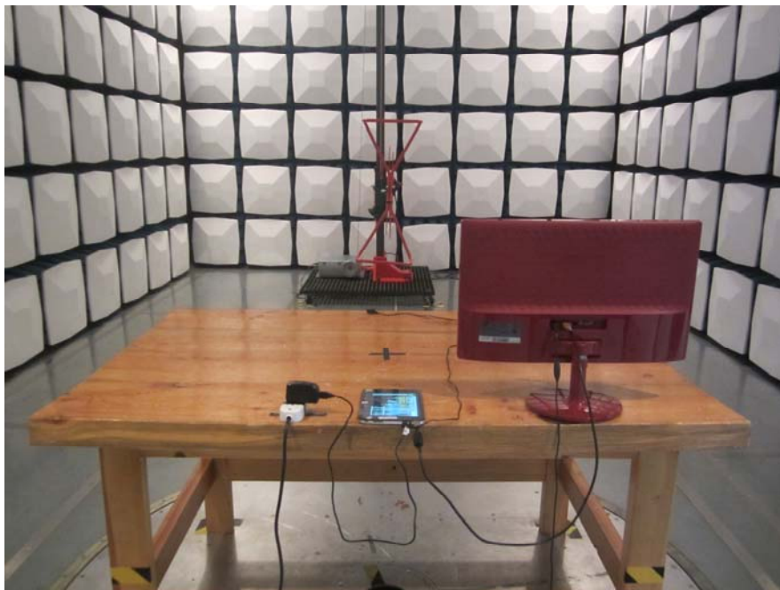
Radiated Emission Below 1GHz Rear View (Charging&Playing Mode)
