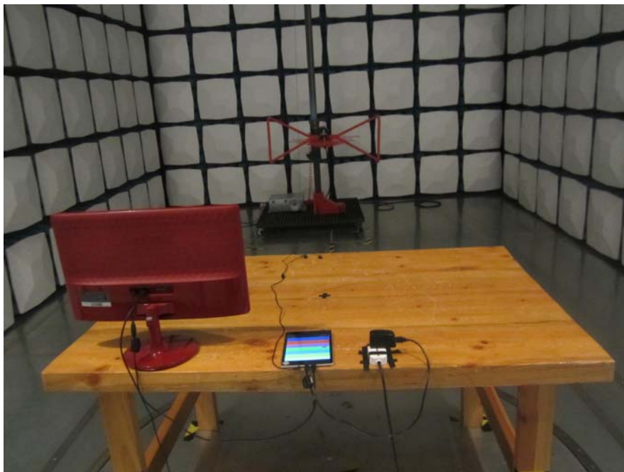
Radiated Emission - Rear View (HDMI Output) (Below 1GHz)
