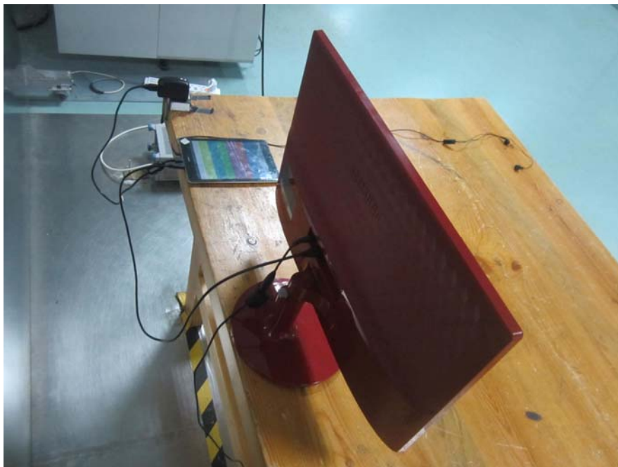
Conducted Emissions – Side View (HDMI Output)
