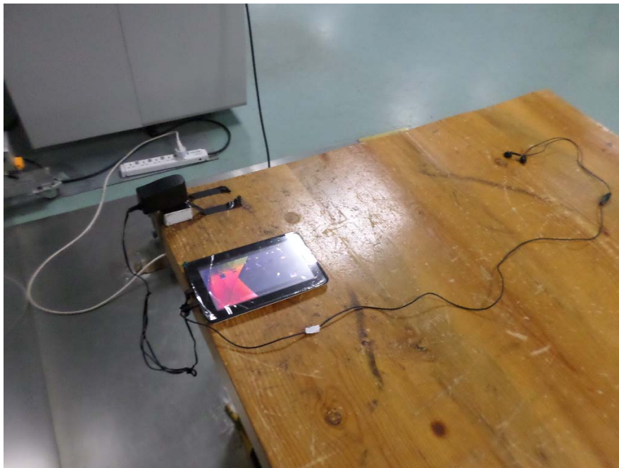
Conducted Emissions –Side View (Charging&Video playing)
