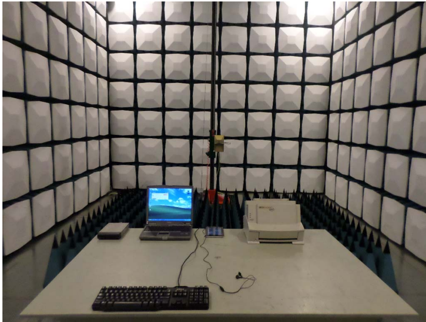
Radiated Emission Above 1GHz -Front View (Downloading)
