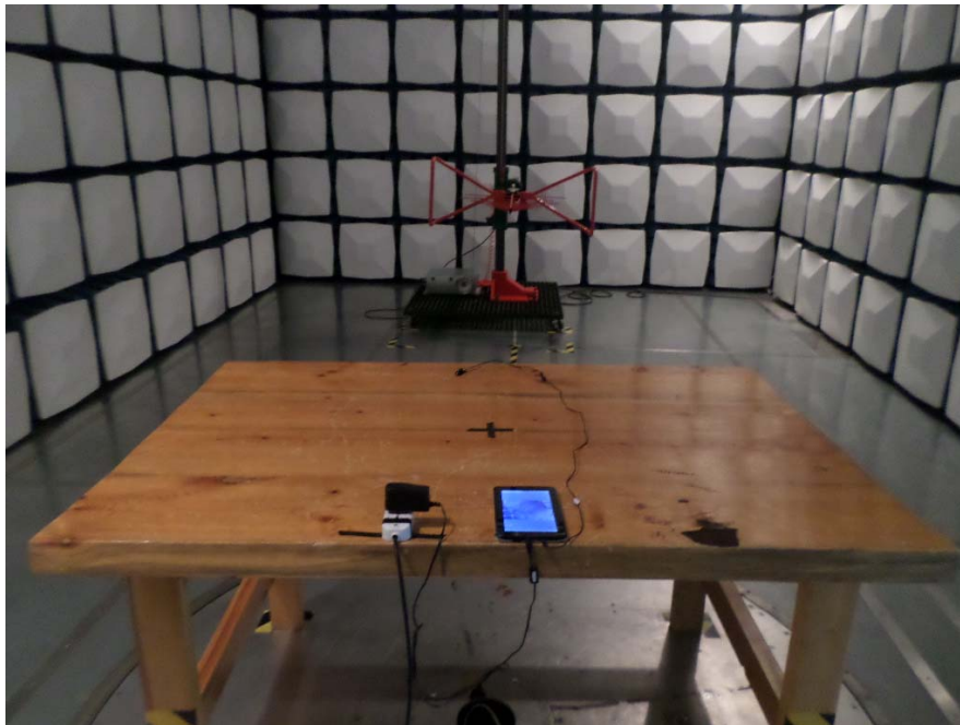
Radiated Emission Below 1GHz - Rear View (Charging&Video playing)
