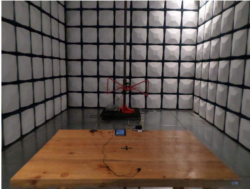
Radiated Emission Below 1GHz -Front View (Charging&Video playing)
