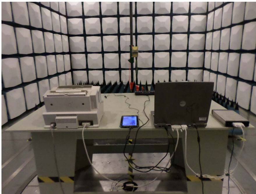
Radiated Emission Above 1GHz- Rear View (Downloading)
