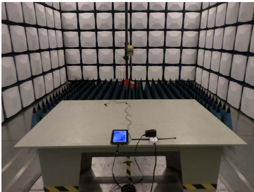
Radiated Emission Above 1GHz- Rear View(Charging&Video playing)
