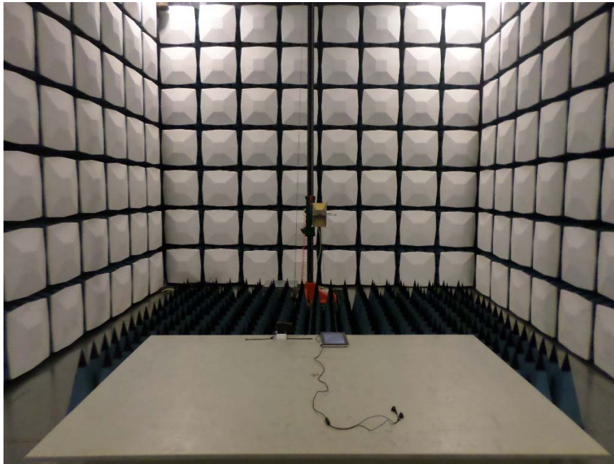
Radiated Emission Above 1GHz -Front View (Charging&Video playing)
