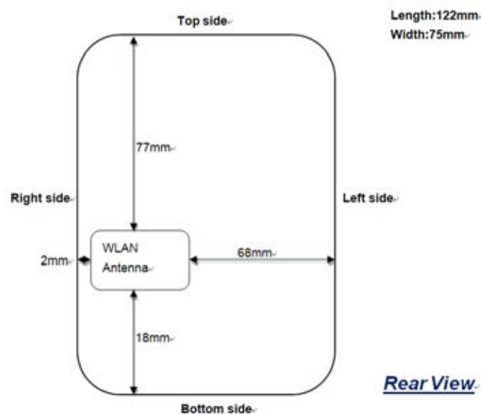
Figure 2: The antenna positions of the DUT
