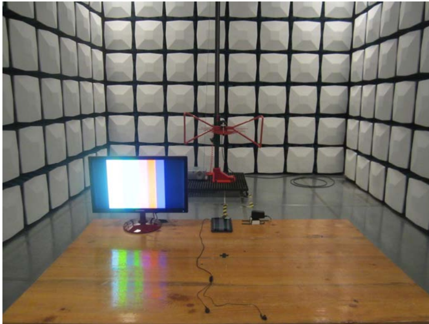
Radiated Emission -Front View (HDMI Output) (Below 1GHz)
