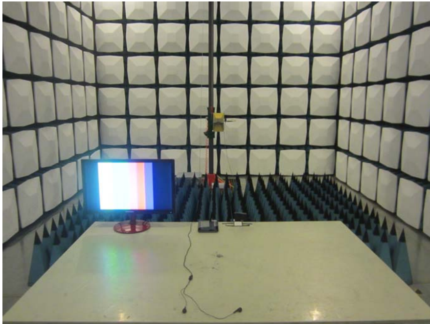
Radiated Emission -Front View (HDMI Output) (Above 1GHz)
