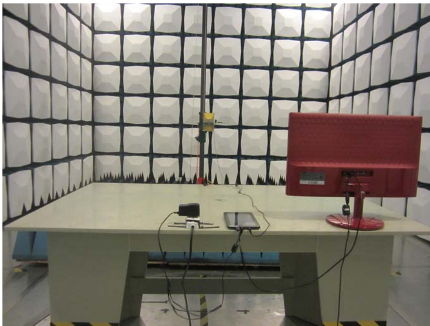
Radiated Emission - Rear View (HDMI Output) (Above 1GHz)
