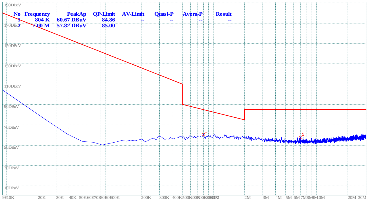
(Plot B.0: 9kHz to 30MHz @ 11/4-DQPSK, channel 39)
