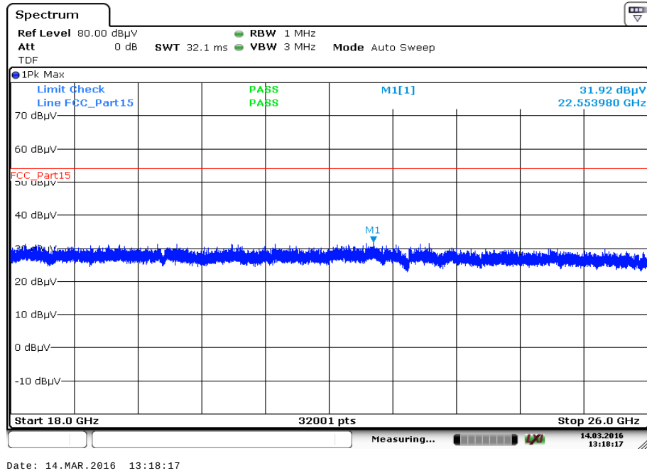
Plot 9: 18 GHz to 26 GHz, TX mode, 2478.5 MHz, vertical & horizontal polarization
