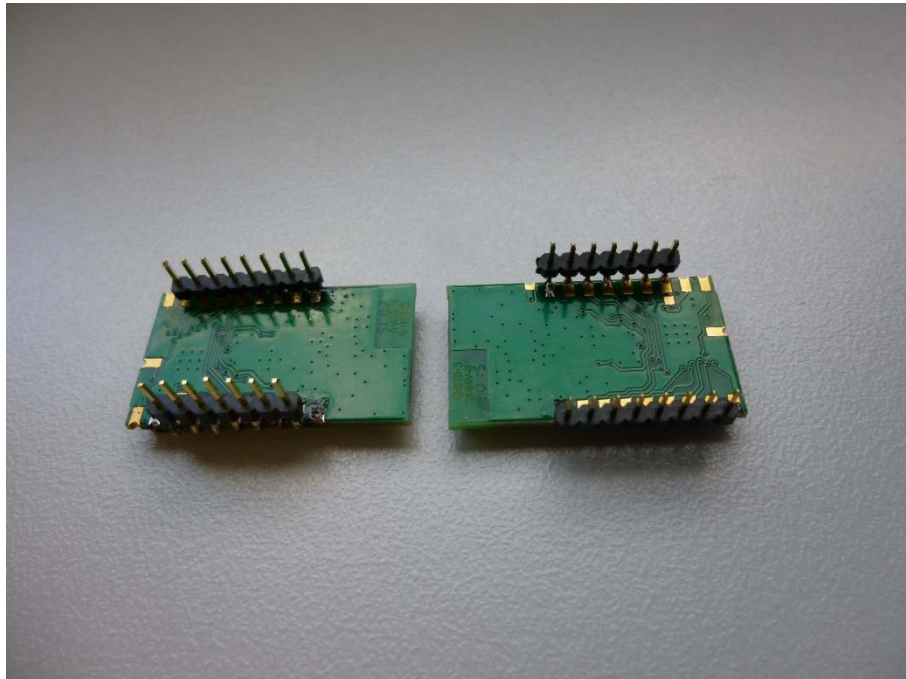
Photo 2: EUT's with UFL connector (left) and ceramic chip antenna (right)
