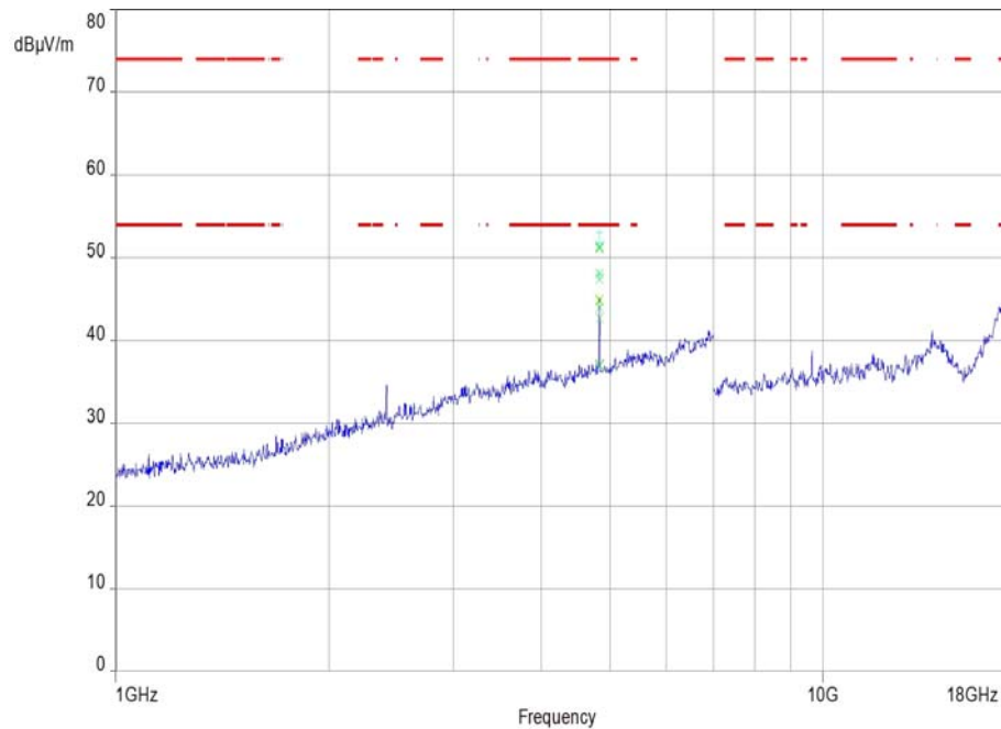
Plot 1: Lowest channel, 1 GHz to 18 GHz, vertical & horizontal polarization
