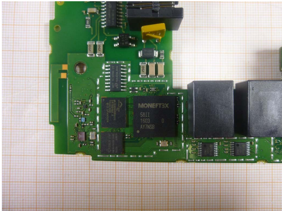
Photo 4: PCB top side view
