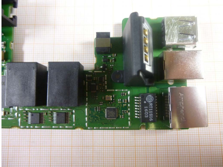
Photo 5: PCB top side view
