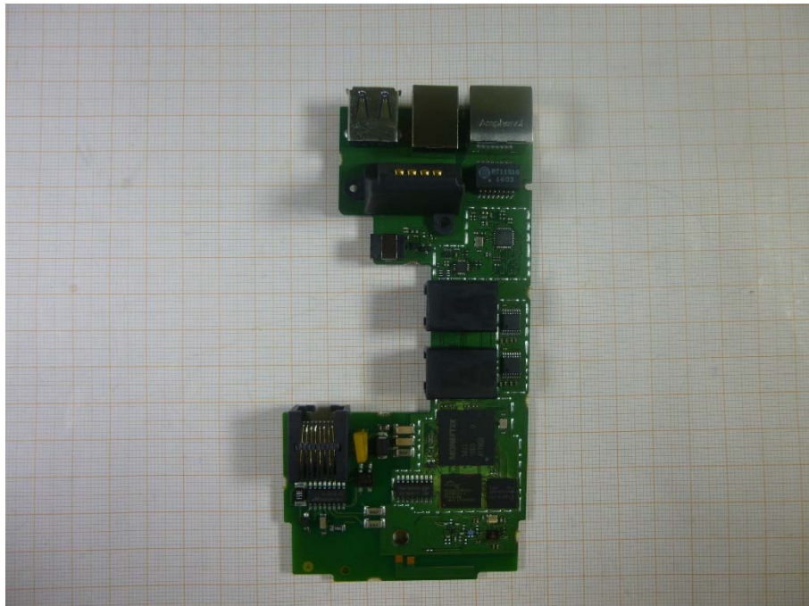
Photo 2: PCB top side view
