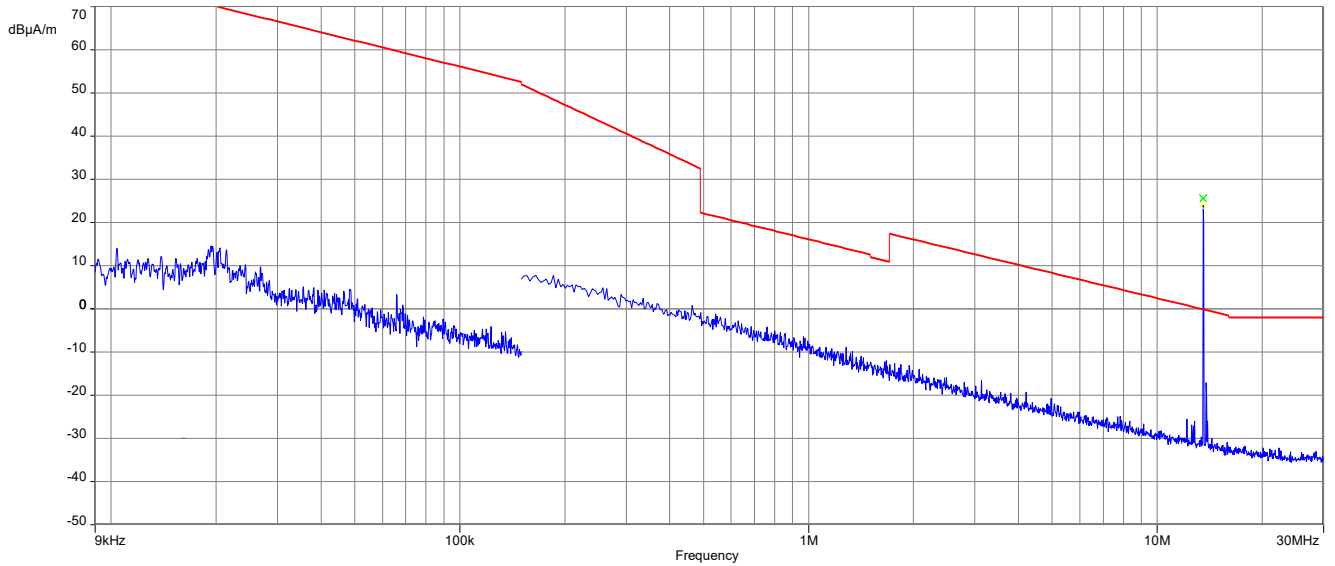
Plot 1: 9 kHz – 30 MHz, magnetic emissions IC
