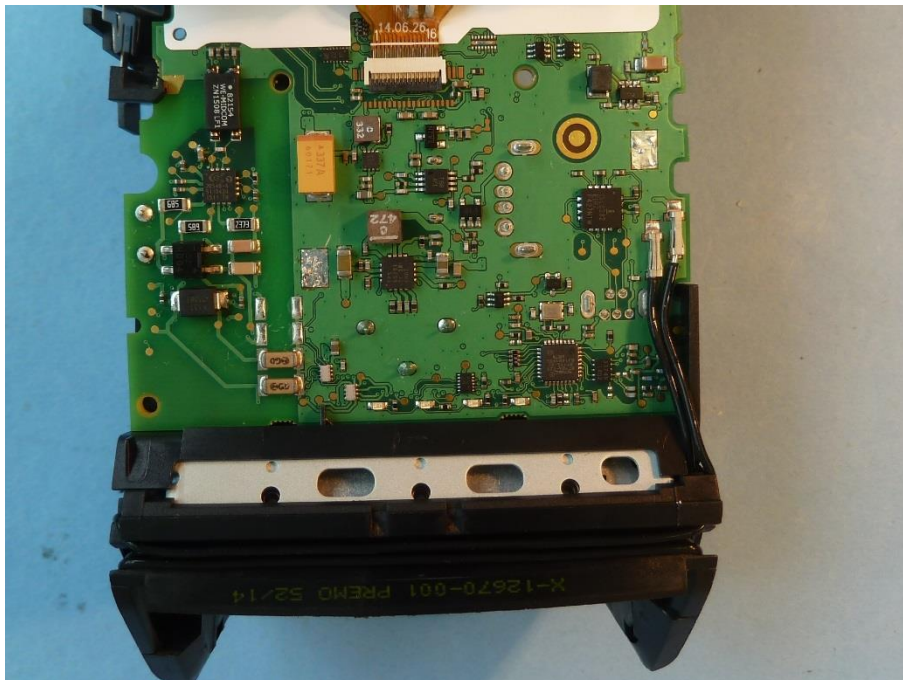
Photo 9: electronic below display
