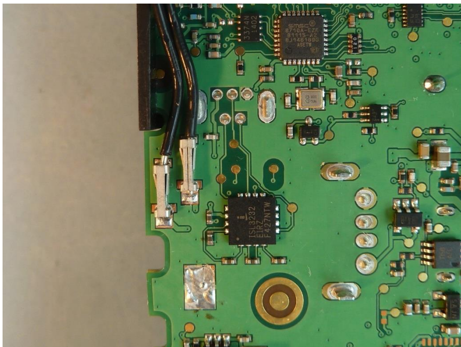
Photo 10: antenna ports
