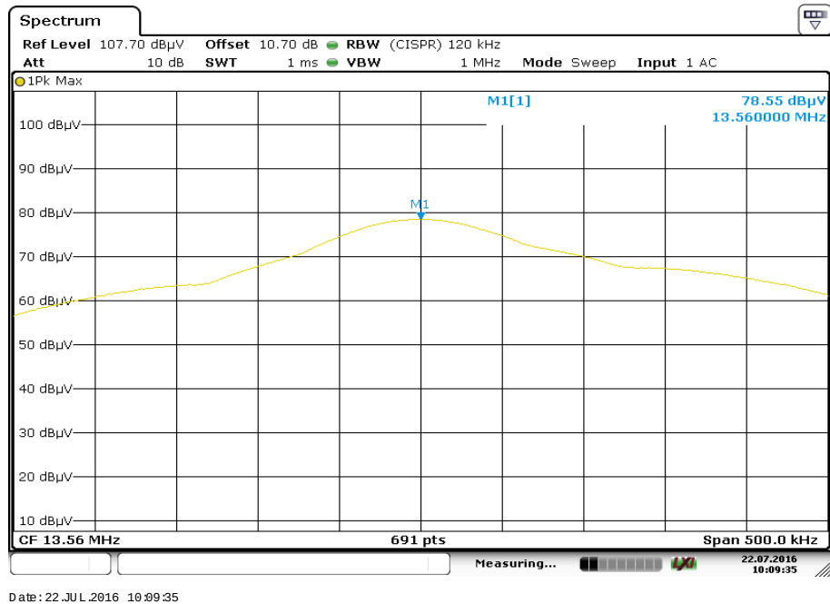
Plot 1: field strength peak
