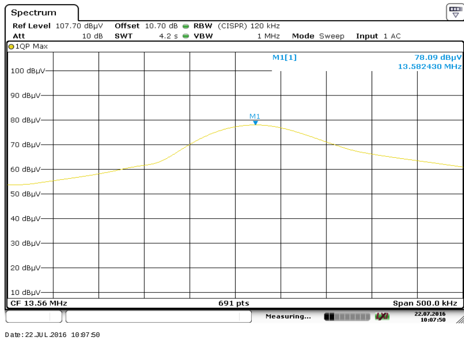
Plot 2: field strength quasi peak
