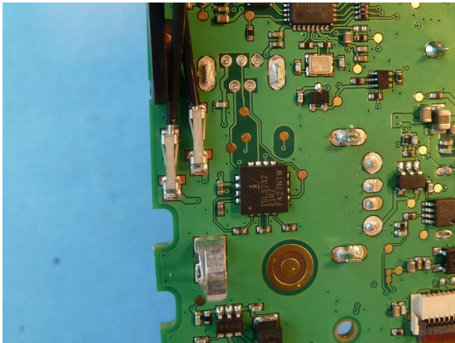
Photo 11: antenna ports
