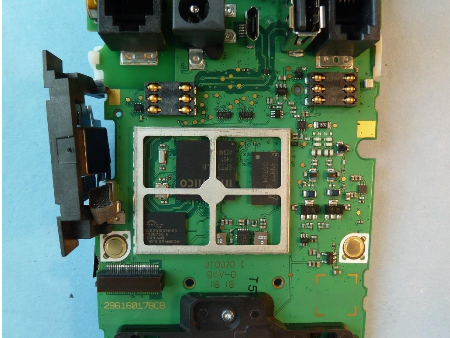
Photo 9: electronic without shielding
