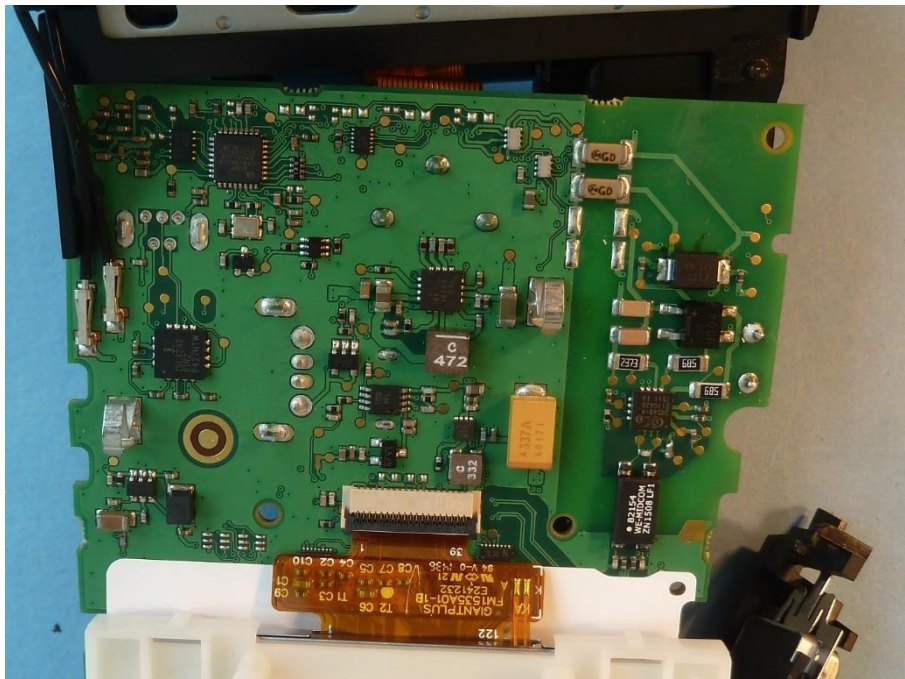
Photo 10: electronic below display
