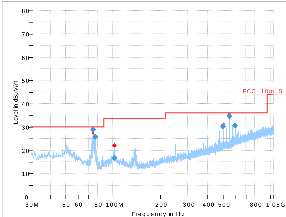
Plot 33: 30 MHz to 1 GHz; vertical & horizontal polarization; U-NII-3; highest channel
