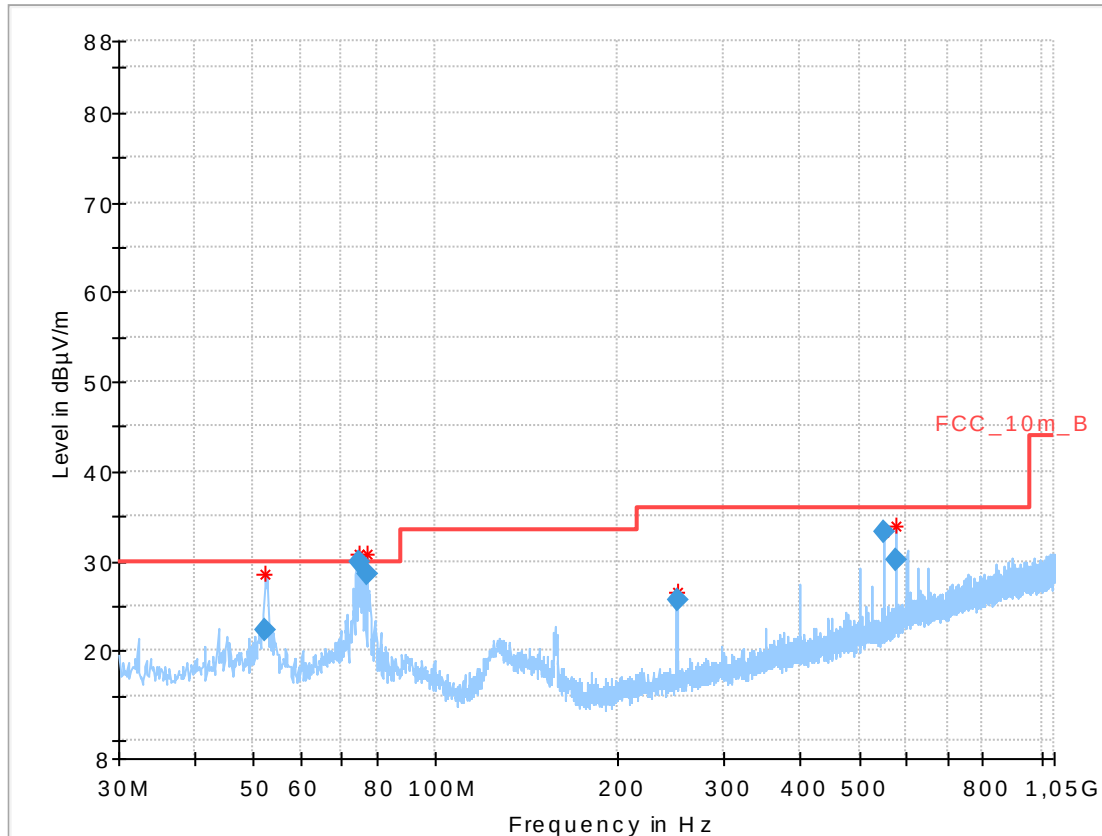
Plot 5: 30 MHz to 1 GHz; vertical & horizontal polarization; U-NII-1; highest channel
