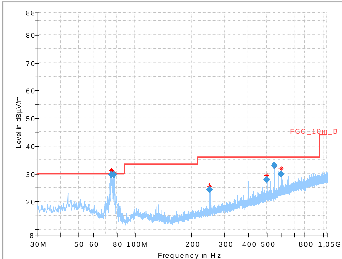
Plot 17: 30 MHz to 1 GHz; vertical & horizontal polarization; U-NII-2C; lowest channel
