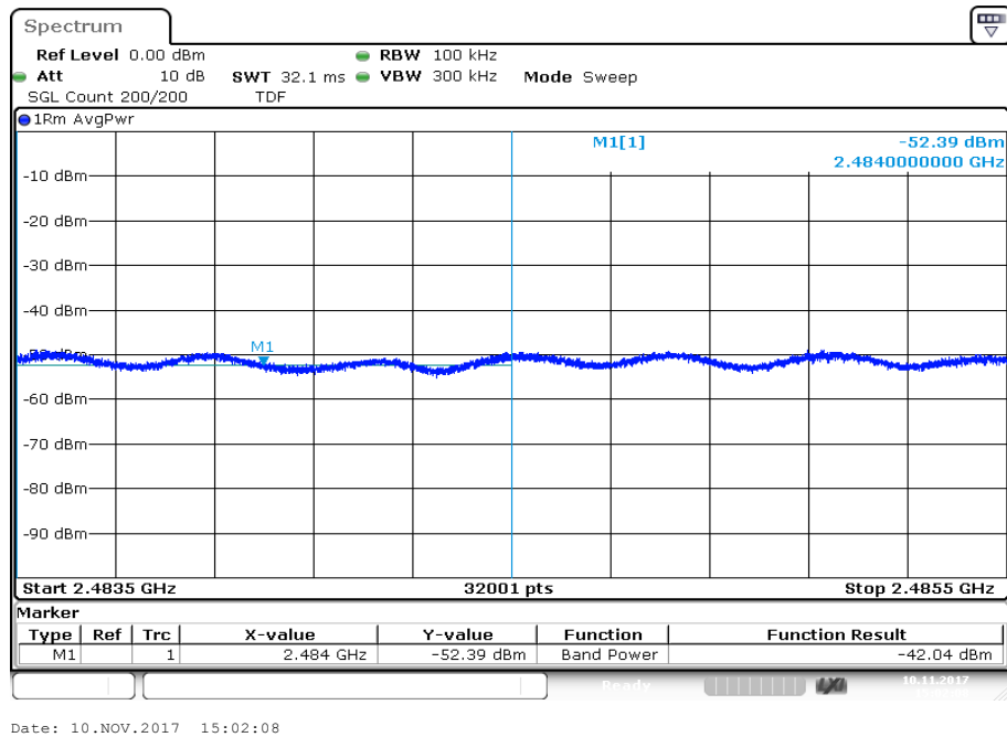
Plot 4: Upper band edge , channel 8
