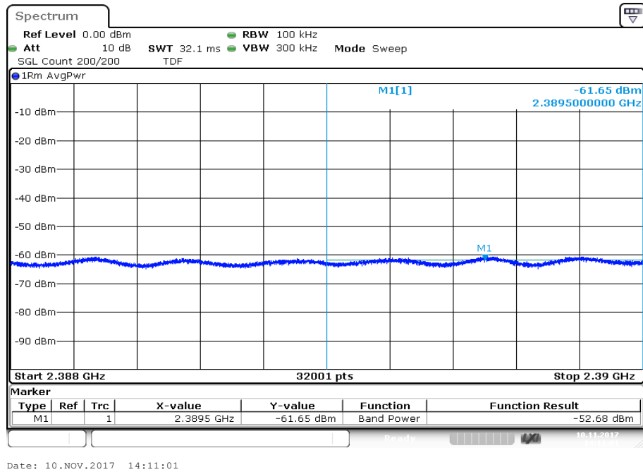
Plot 3: Lower band edge, channel 4
