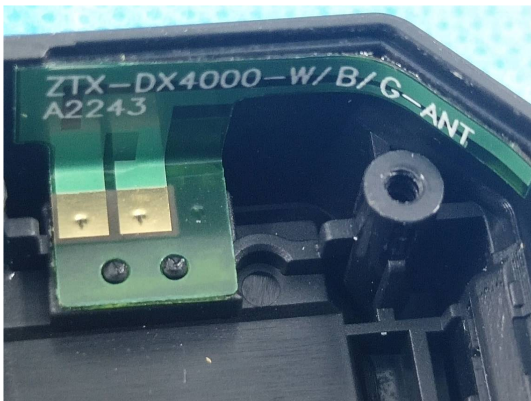
WiFi/BT Antenna
