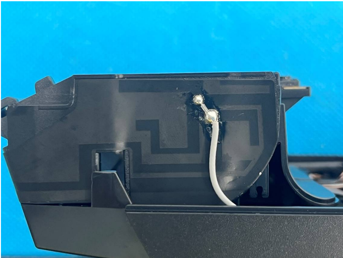
GSM/WCDMA/LTE Main Antenna
