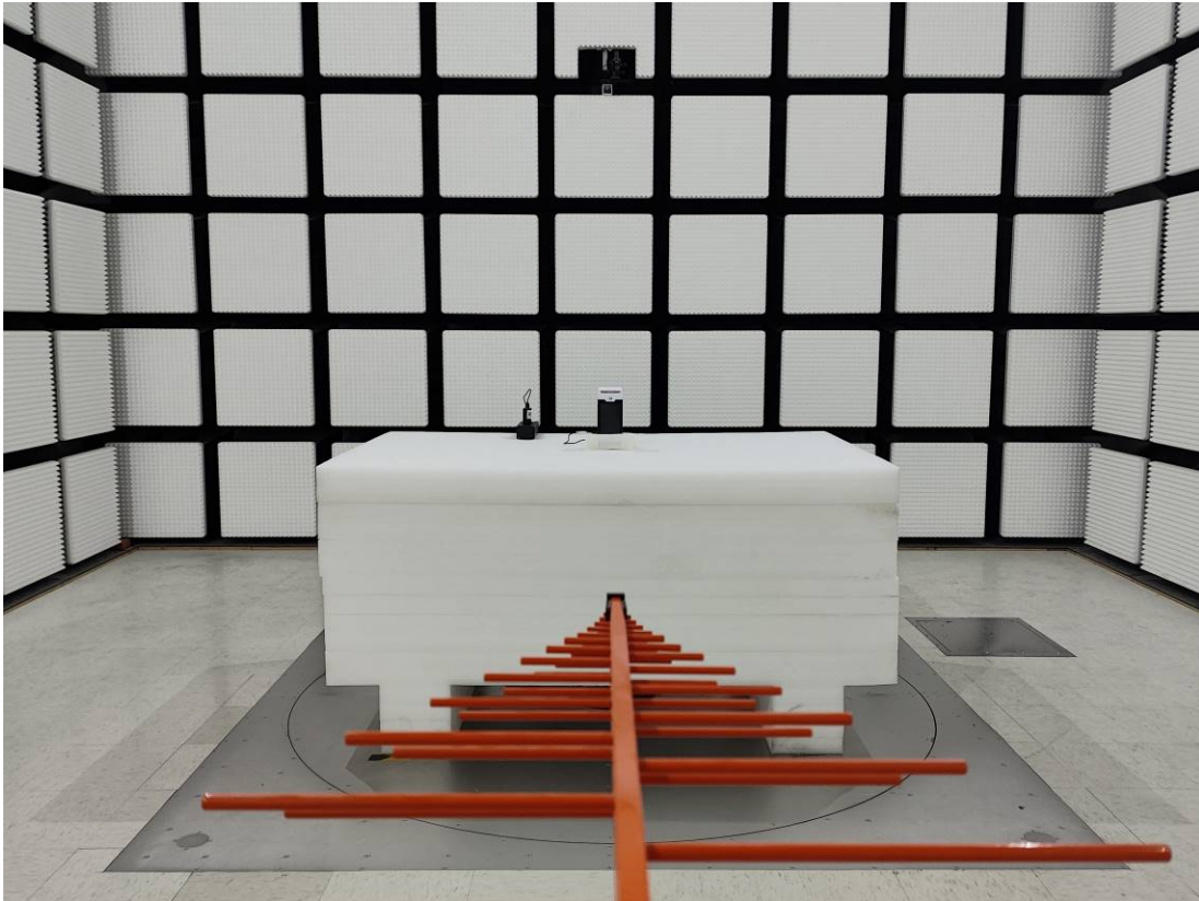
Radiated Emission Above 1GHz View-Adapter 4#
