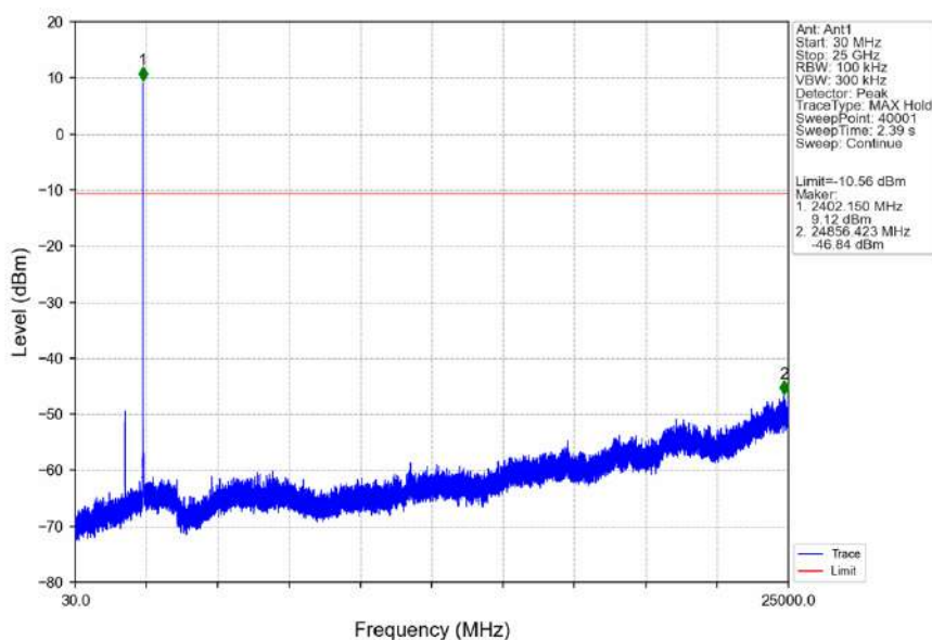
GFSK_DH5_LCH_2402MHz_Ant1_NTNV
