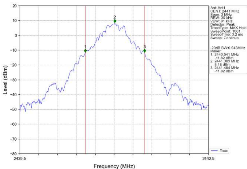
GFSK_DH5_MCH_2441MHz_Ant1_NTNV
