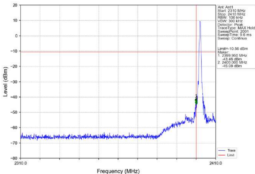
GFSK_DH5_LCH_2402MHz_Ant1_NTNV
