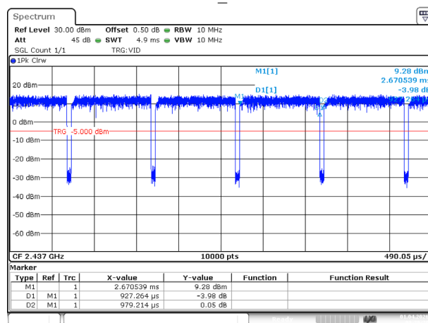
802.11n40_2437MHz
