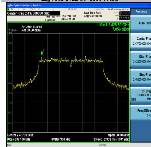
11g-Ant1-2437-0-Reference-PASS
