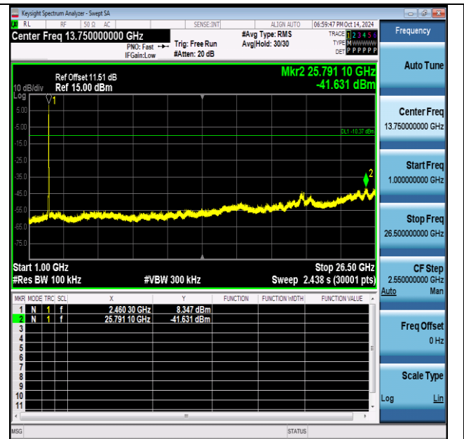
11g-Ant1-2462-1000~26500-PASS
