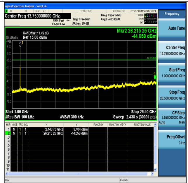
11n20SISO-Ant1-2437-1000~26500-PASS
