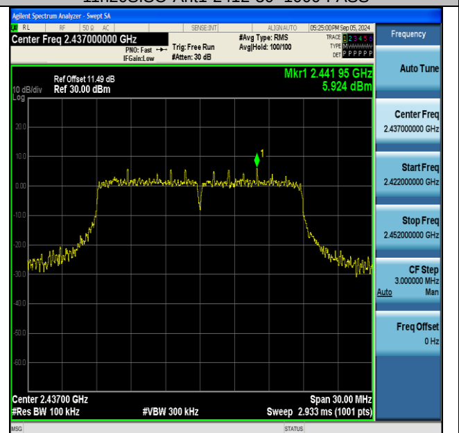
11n20SISO-Ant1-2437-0~Reference-PASS
