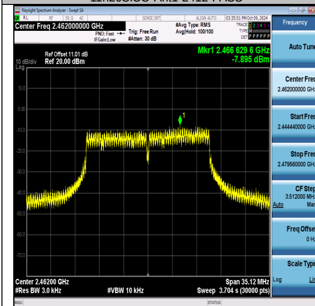
11n20SISO-Ant1-2462-PASS
