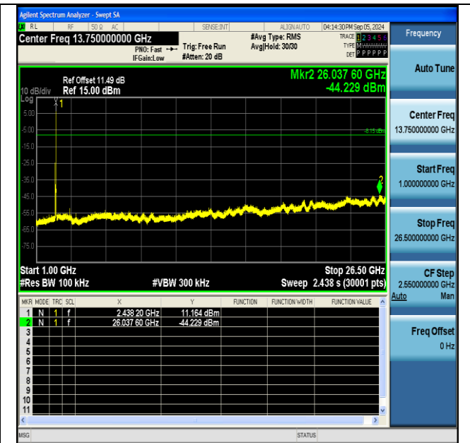
11b-Ant1-2437-1000~26500-PASS
