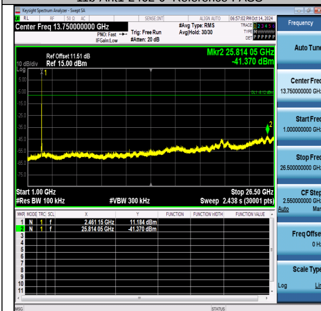
11b-Ant1-2462-1000~26500-PASS
