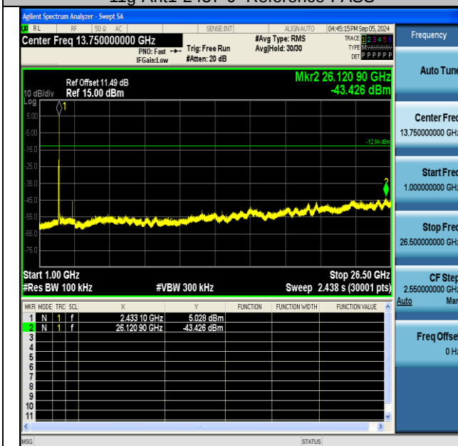
11g-Ant1-2437-1000~26500-PASS
