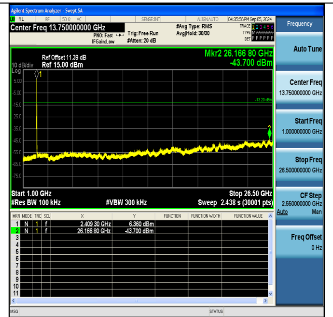
11g-Ant1-2412-1000~26500-PASS
