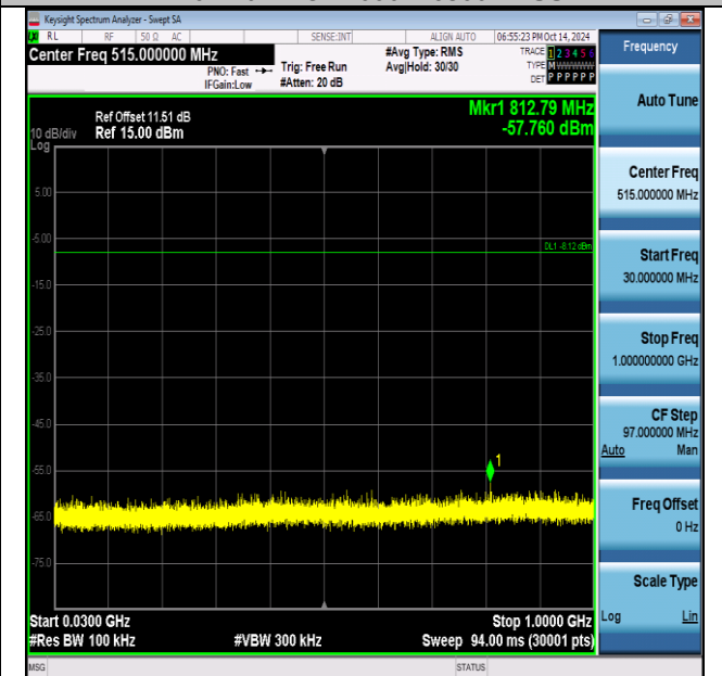
11b-Ant1-2462-30~1000-PASS
