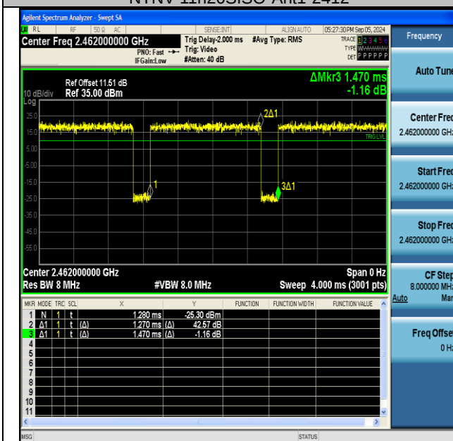
NTNV-11n20SISO-Ant1-2462
