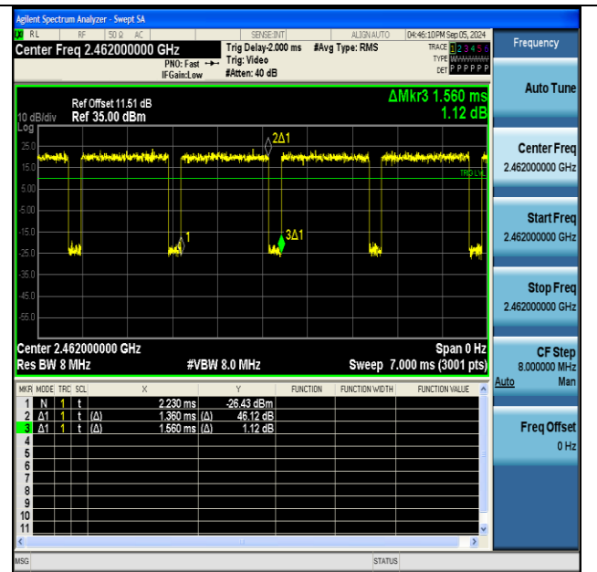
NTNV-11g-Ant1-2462
