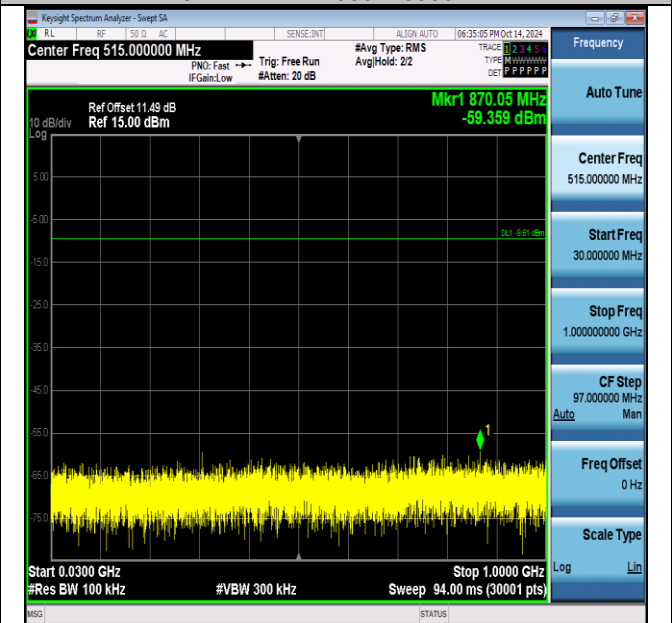
DH5-Ant1-2480-30~1000-PASS
