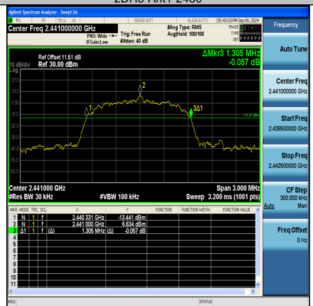
3DH5-Ant1-2441
