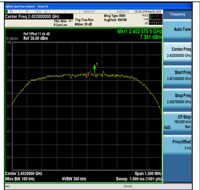
2DH5-Ant1-2402-0~Reference-PASS
