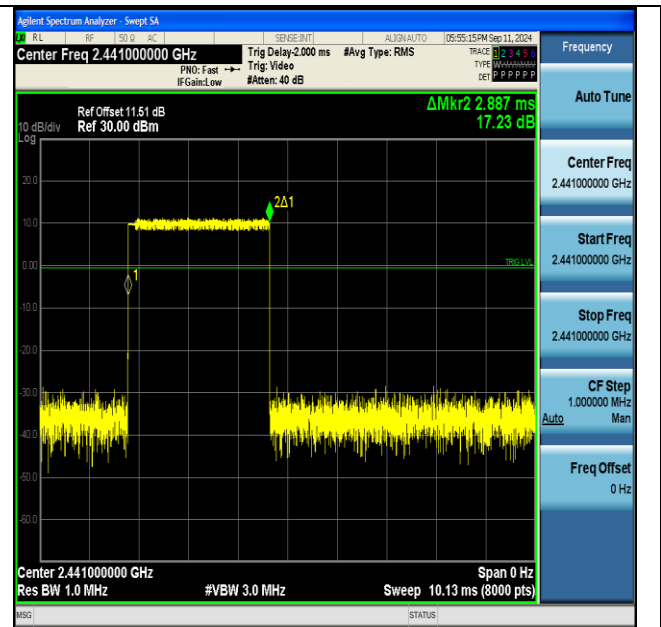
2DH5-Ant1-Hop-PASS
