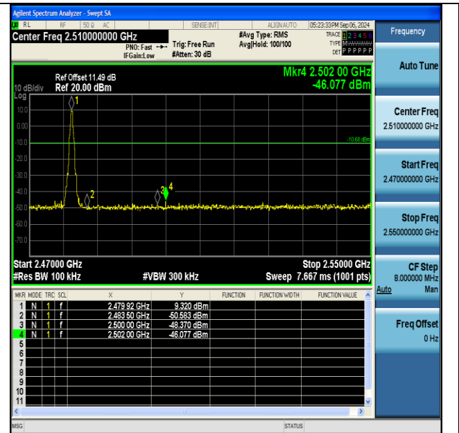
DH5-Ant1-2480-PASS
