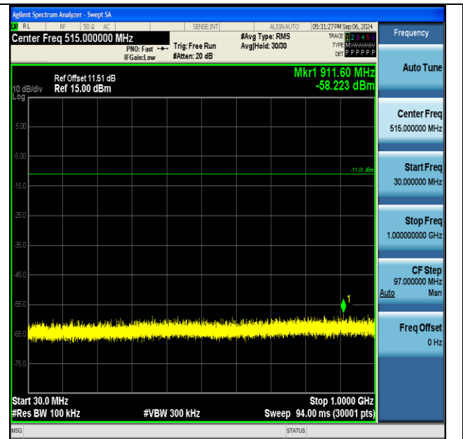
2DH5-Ant1-2441-30~1000-PASS
