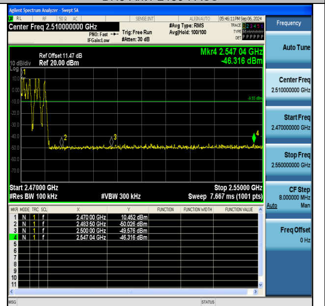
DH5-Ant1-Hop_2480-PASS
