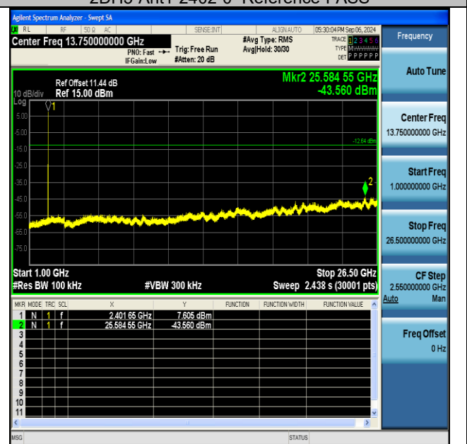
2DH5-Ant1-2402-1000~26500-PASS
