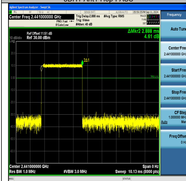
3DH5-Ant1-Hop-PASS
