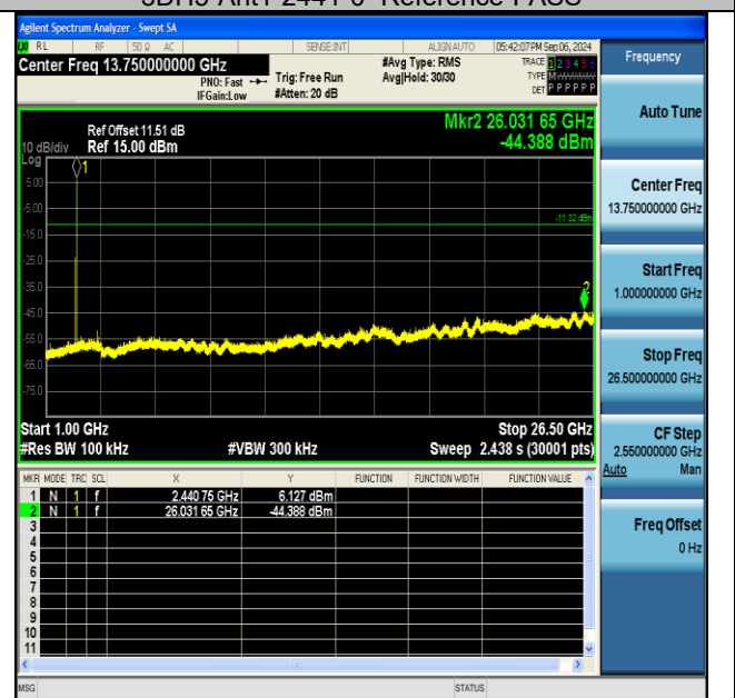
3DH5-Ant1-2441-1000~26500-PASS
