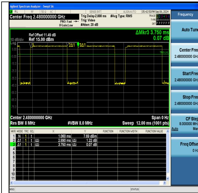
NTNV-3DH5-Ant1-2480
