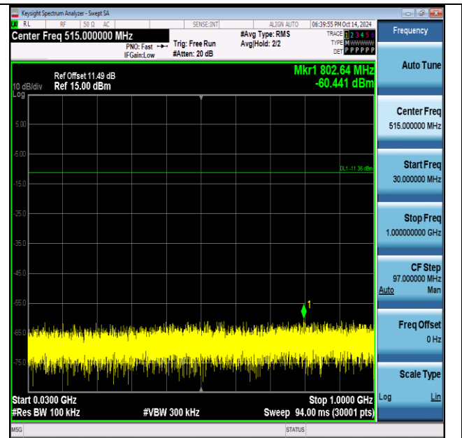
3DH5-Ant1-2480-30~1000-PASS
