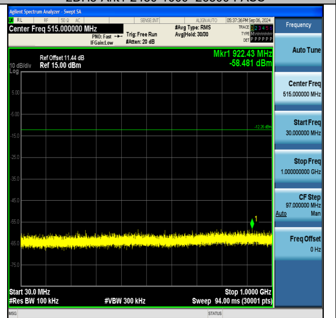
3DH5-Ant1-2402-30~1000-PASS
