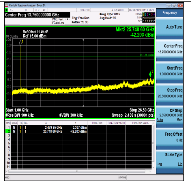
2DH5-Ant1-2480-1000~26500-PASS
