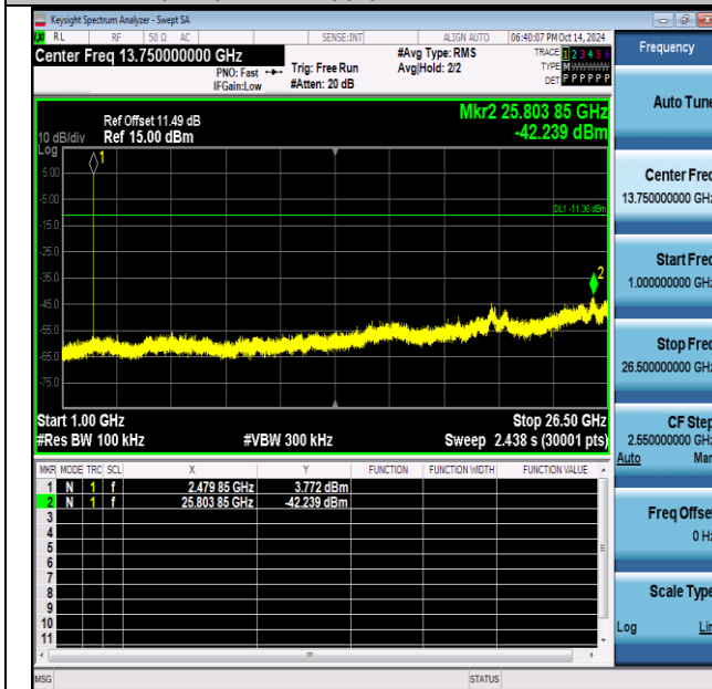
3DH5-Ant1-2480-1000~26500-PASS
