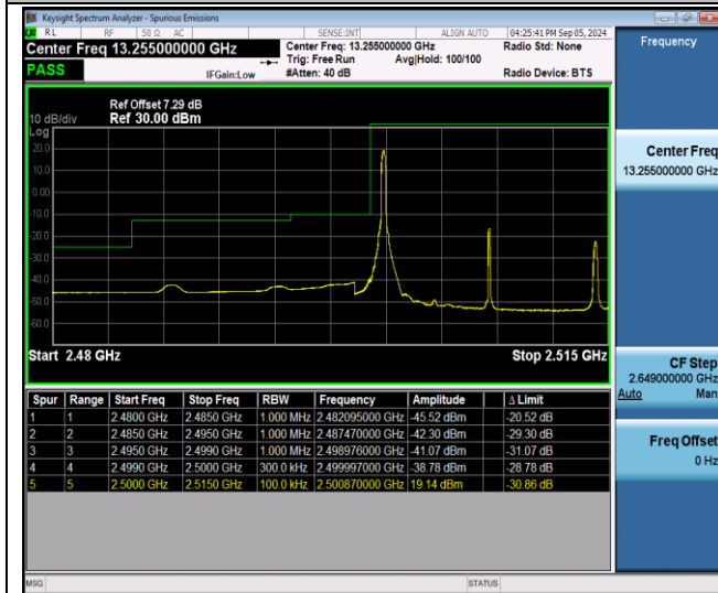
Band7-15MHz-QPSK-20825-1RB#0-PASS
