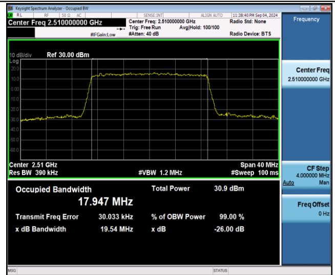
Band7-20MHz-16QAM-20850-100RB#0-PASS
