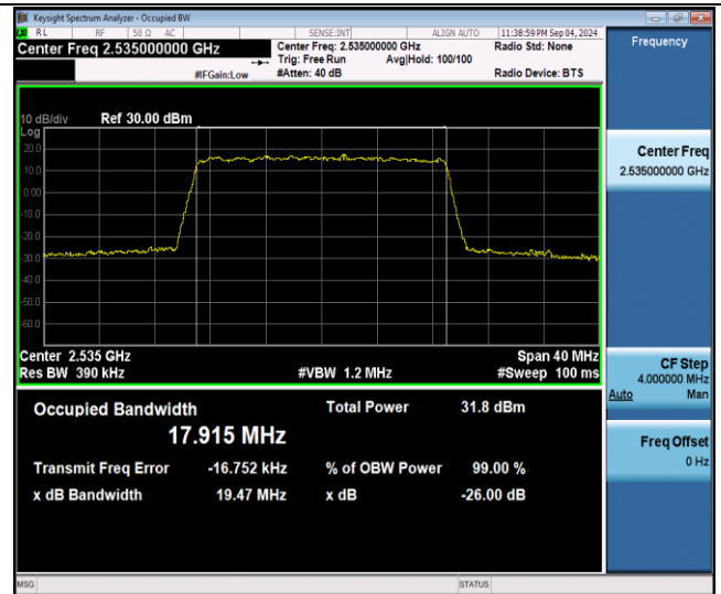
Band7-20MHz-QPSK-21100-100RB#0-PASS
