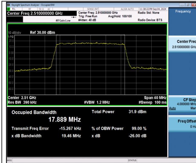
Band7-20MHz-QPSK-20850-100RB#0-PASS
