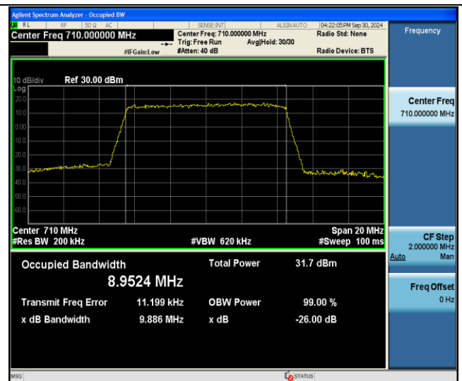
Band17-10MHz-QPSK-23790-50RB#0-PASS
