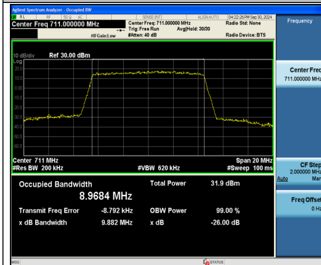
Band17-10MHz-QPSK-23800-50RB#0-PASS
