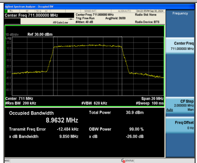
Band17-10MHz-16QAM-23800-50RB#0-PASS
