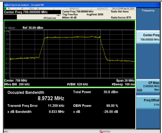
Band17-10MHz-16QAM-23780-50RB#0-PASS
